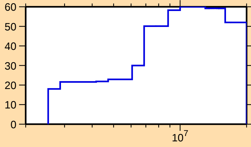
\Delta\sigma/\sigma vs. E for ^{226}\text{Rn}(n,\text{inel.})
