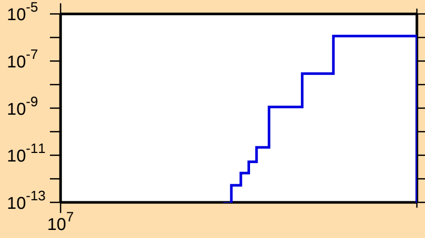
\sigma vs. E for ^{226}\text{Rn}(n,nt)
