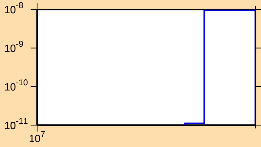
\sigma vs. E for ^{226}\text{Rn}(n,\text{nd})
