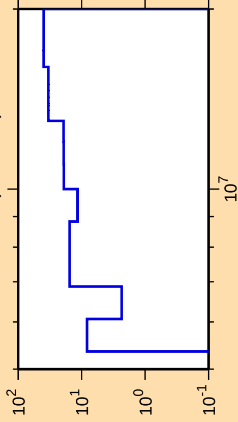
\Delta\sigma/\sigma vs. E for ^{226}\text{Rn}(n,n\text{cont.})
