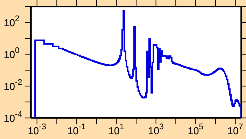
\sigma vs. E for ^{226}\text{Rn}(n,\gamma)
