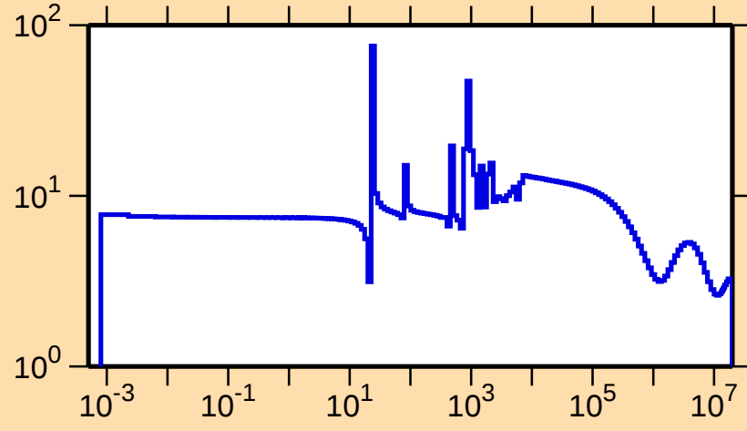
\sigma vs. E for ^{226}\text{Rn}(n,\text{el.})
