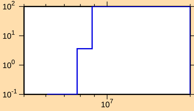
\Delta\sigma/\sigma vs. E for ^{226}\text{Rn}(n,p)
