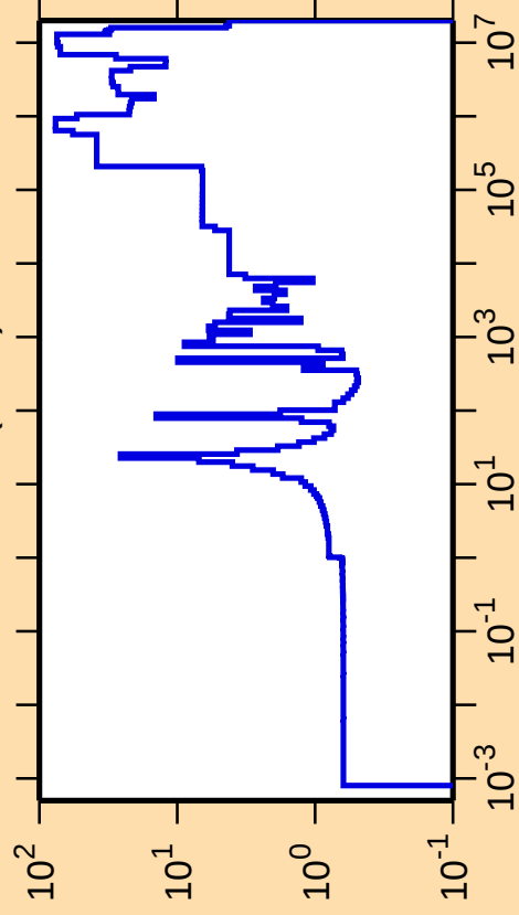
\Delta\sigma/\sigma vs. E for ^{226}\text{Rn}(n,\text{el.})
