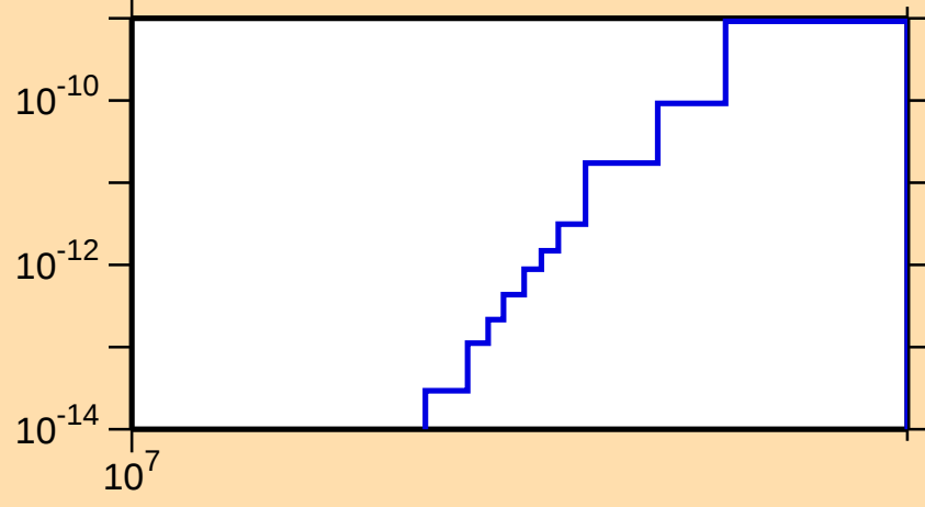
\sigma vs. E for ^{226}\text{Rn}(n,3n\alpha)
