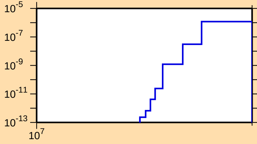
\sigma vs. E for ^{227}\text{Rn}(n,nt)
