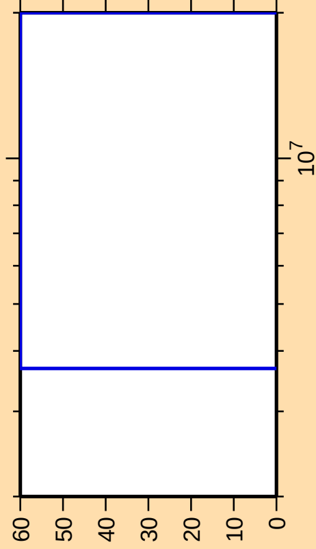
\Delta\sigma/\sigma vs. E for ^{227}\text{Rn}(n,\gamma)
