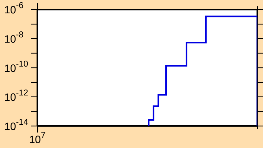
\sigma vs. E for ^{227}\text{Rn}(n,\text{nd})
