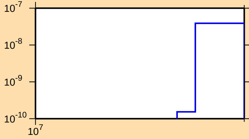
\sigma vs. E for ^{227}\text{Rn}(n,2np)
