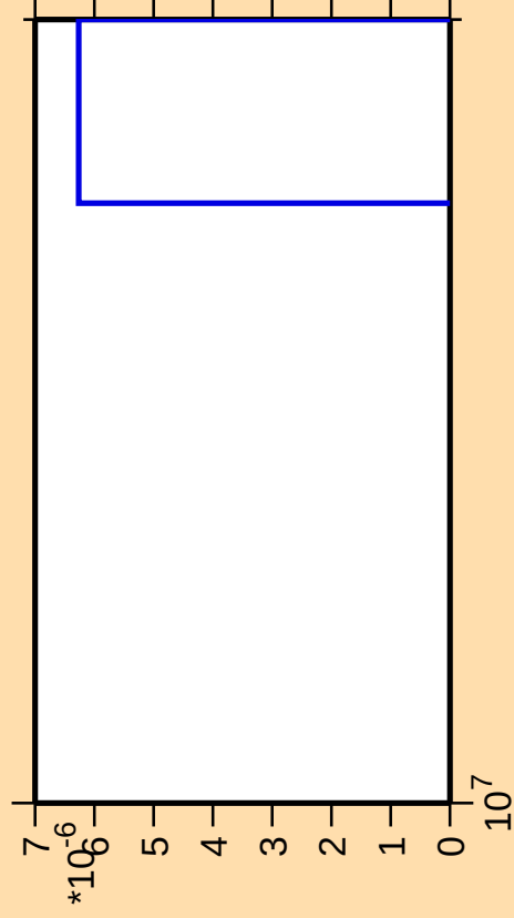
\Delta\sigma/\sigma vs. E for ^{227}\text{Rn} (mt 42)
