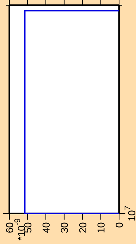
\Delta\sigma/\sigma vs. E for ^{227}\text{Rn}(\text{mt } 42)
