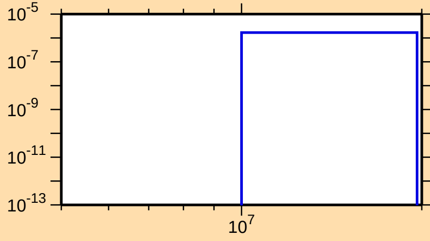
\sigma vs. E for ^{227}\text{Rn}(n,np)
