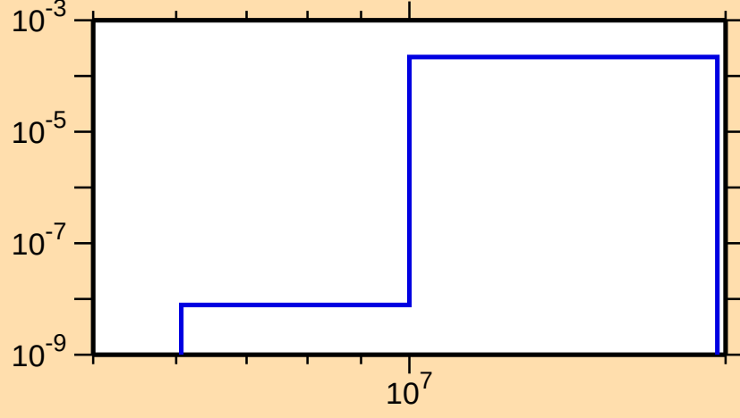
\sigma vs. E for ^{227}\text{Rn}(n,p)
