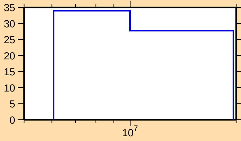
\Delta\sigma/\sigma vs. E for ^{227}\text{Rn}(n,\text{tot.})
