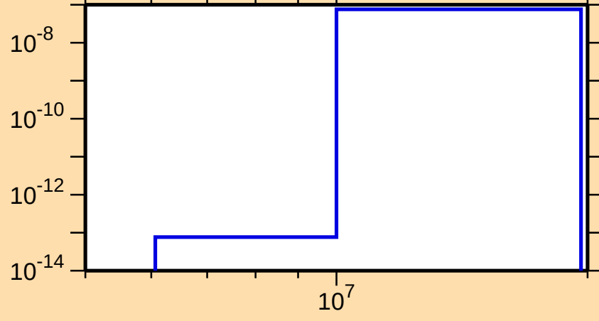
\sigma vs. E for ^{227}\text{Rn}(n,2n\alpha)
