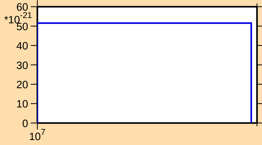
\sigma vs. E for ^{227}\text{Rn}(\text{mt } 42)
