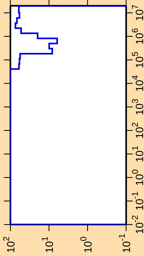
\Delta\sigma/\sigma vs. E for ^{227}\text{Rn}(n,\text{nonel.})
