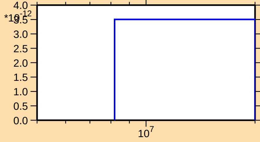
\sigma vs. E for ^{227}\text{Rn}(n,3n\alpha)
