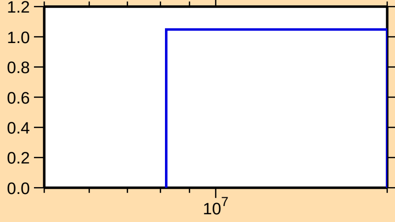
\sigma vs. E for ^{227}\text{Rn}(n,3n)
