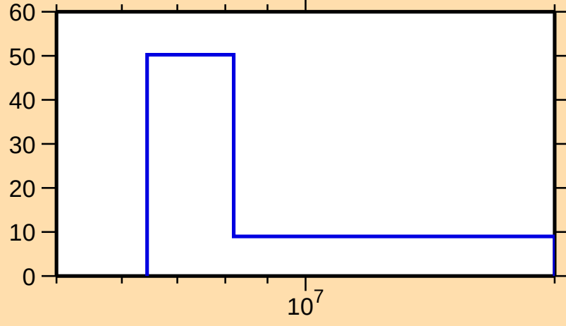
\Delta\sigma/\sigma vs. E for ^{227}\text{Rn}(n,n_1)
