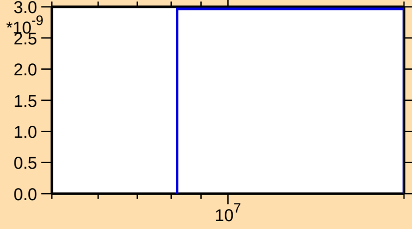
\sigma vs. E for ^{227}\text{Rn}(n,\text{nd})
