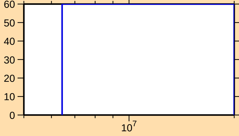
\Delta\sigma/\sigma vs. E for ^{227}\text{Rn}(n,2n)
