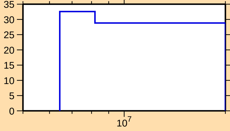
\Delta\sigma/\sigma vs. E for ^{227}\text{Rn}(n,\text{tot.})
