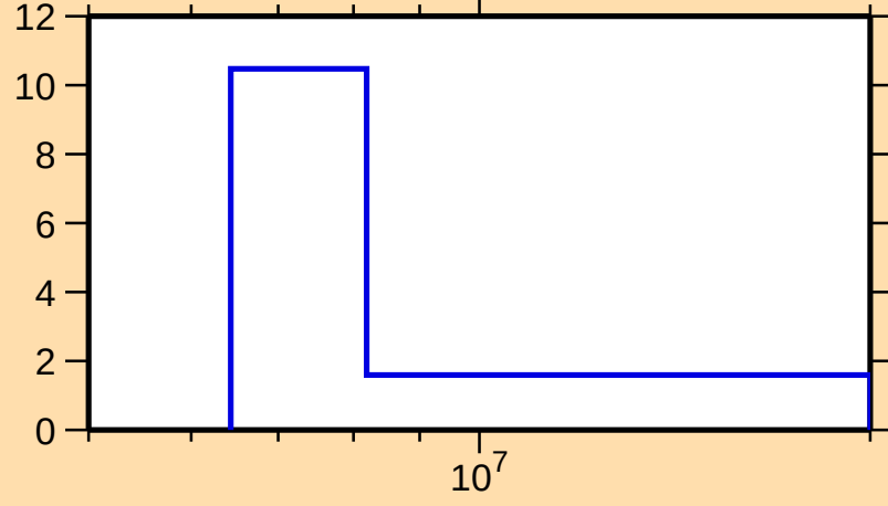
\Delta\sigma/\sigma vs. E for ^{227}\text{Rn}(n,\text{el.})
