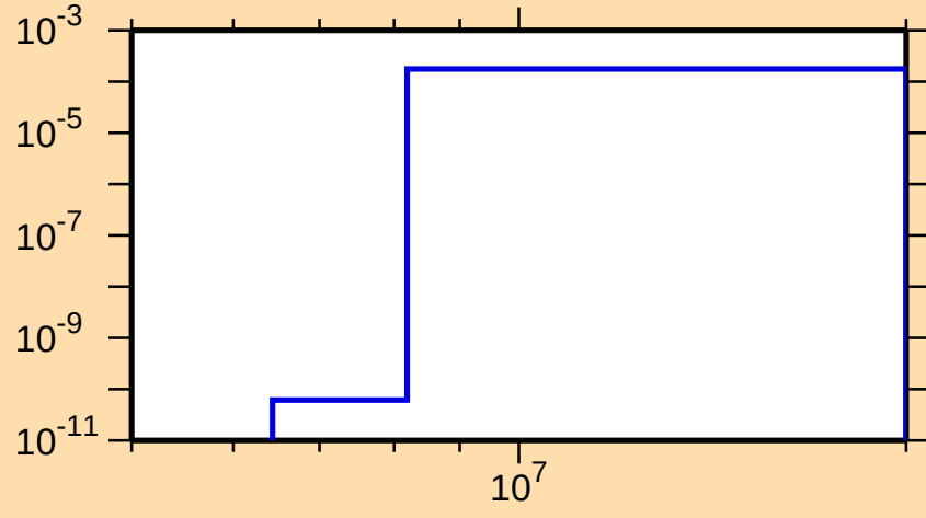
\sigma vs. E for ^{227}\text{Rn}(n,p)
