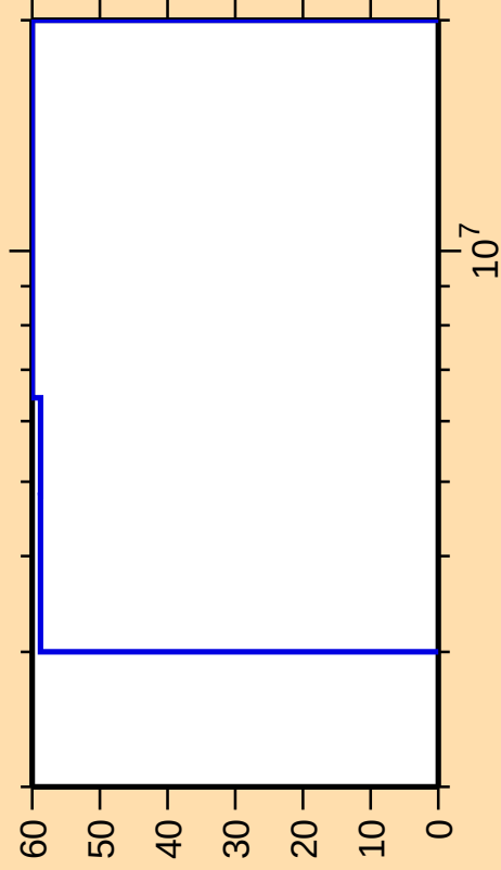
\Delta\sigma/\sigma vs. E for ^{227}\text{Rn}(n,2n)
