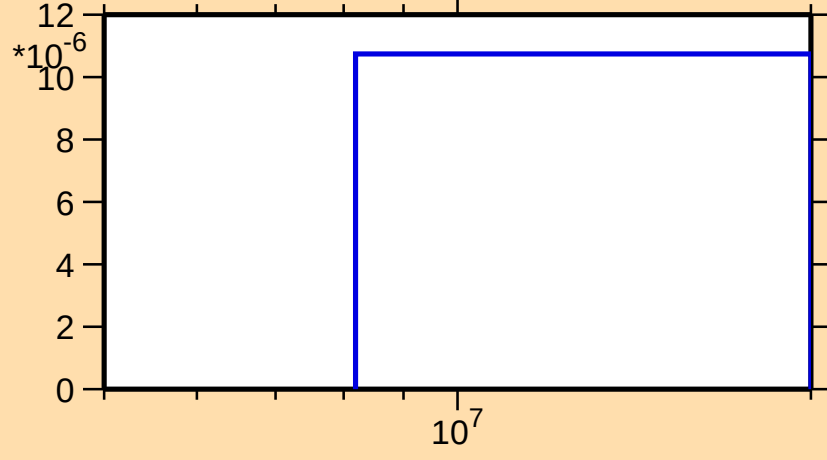
\sigma vs. E for ^{227}\text{Rn}(n,t)
