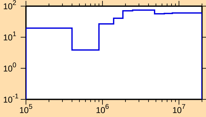
\Delta\sigma/\sigma vs. E for ^{227}\text{Rn}(n,n\text{onel.})
