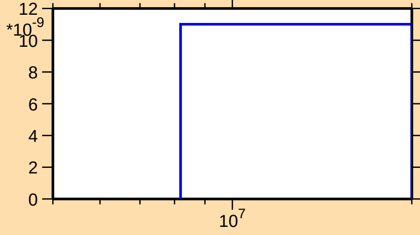
\sigma vs. E for ^{227}\text{Rn}(n,nt)
