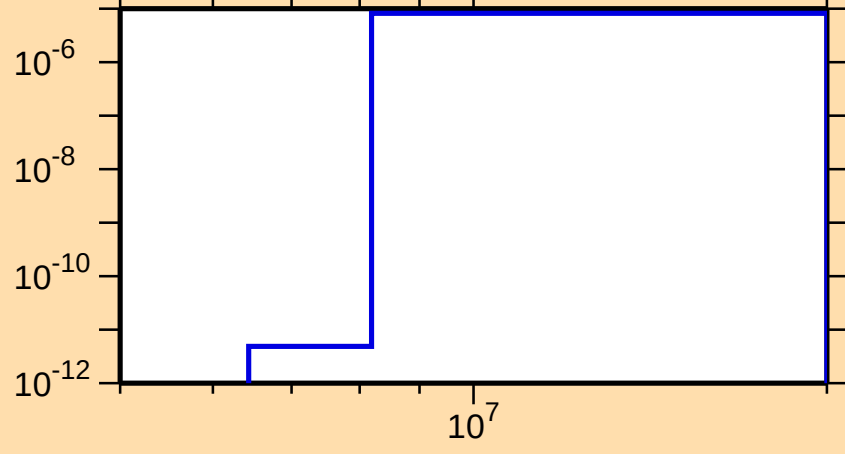
\sigma vs. E for ^{227}\text{Rn}(n,n\alpha)
