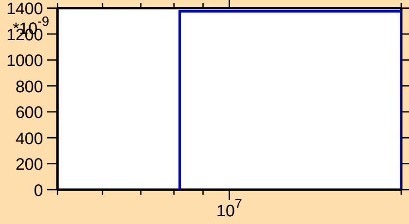
\sigma vs. E for ^{227}\text{Rn}(n,np)
