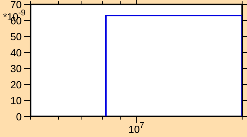
\sigma vs. E for ^{227}\text{Rn}(n,2n\alpha)
