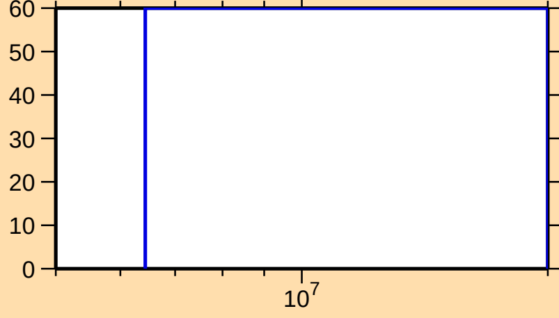
\Delta\sigma/\sigma vs. E for ^{227}\text{Rn}(n,n\text{cont.})
