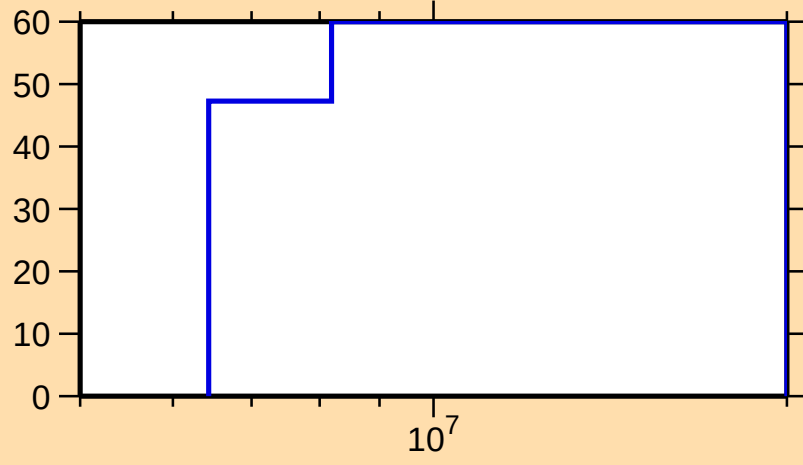
\Delta\sigma/\sigma vs. E for ^{227}\text{Rn}(n,\text{inel.})
