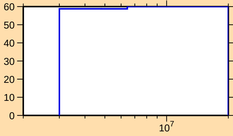
\Delta\sigma/\sigma vs. E for ^{227}\text{Rn}(n,2n)
