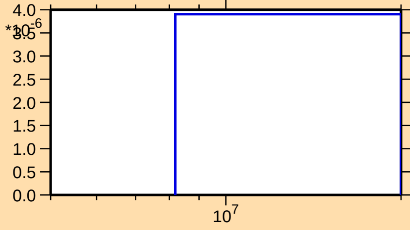
\sigma vs. E for ^{227}\text{Rn}(n,d)
