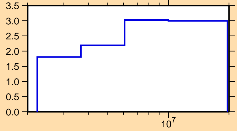
\Delta\sigma/\sigma vs. E for ^{89}\text{Ru}(n,n\text{nonel.})
