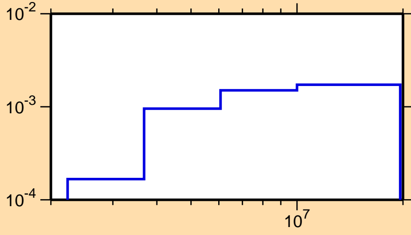
\sigma vs. E for ^{89}\text{Ru}(n,n\text{cont.})
