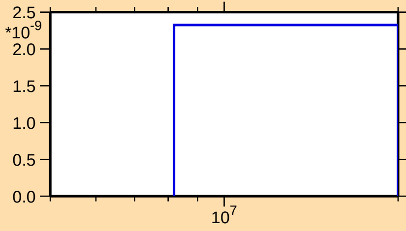
\sigma vs. E for ^{89}\text{Ru}(\text{mt } 45)
