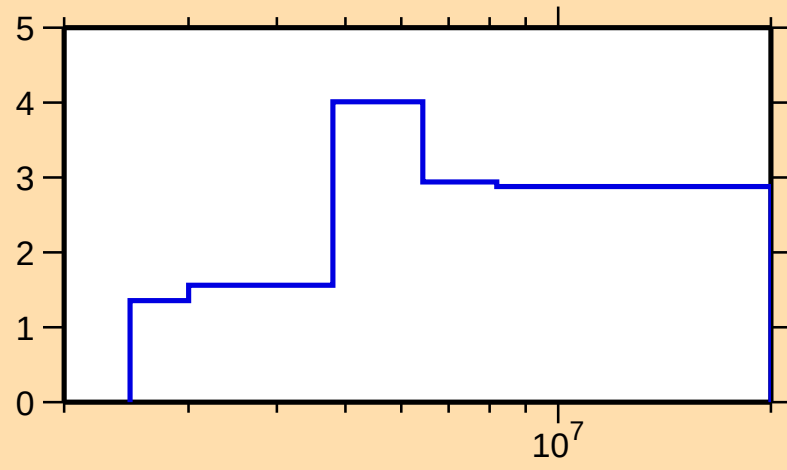
\Delta\sigma/\sigma vs. E for ^{89}\text{Ru}(n,n\text{onel.})
