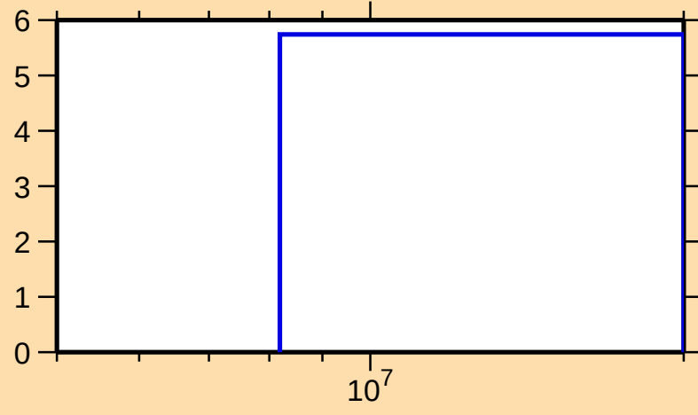
\Delta\sigma/\sigma vs. E for ^{89}\text{Ru}(n,\text{el.})
