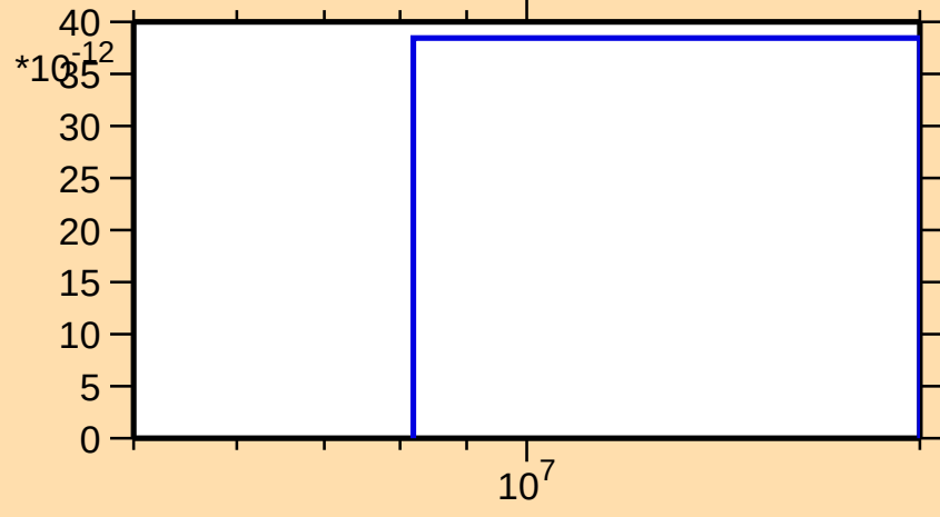
\sigma vs. E for ^{89}\text{Ru}(\text{mt117})
