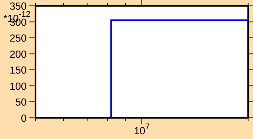
\sigma vs. E for ^{89}\text{Ru}(\text{mt } 34)
