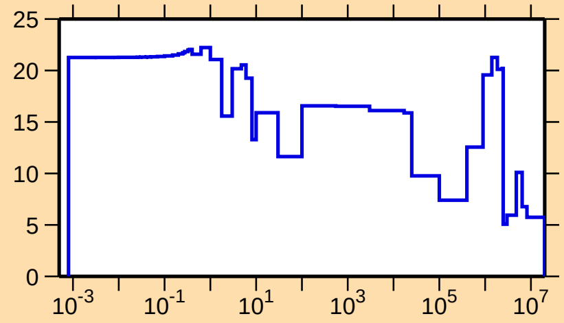
\Delta\sigma/\sigma vs. E for ^{89}\text{Ru}(n,\text{el.})
