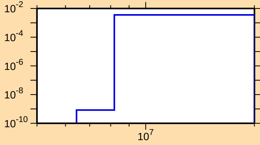
\sigma vs. E for ^{89}\text{Ru}(n,\text{pd})
