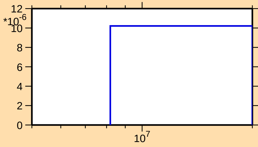
\sigma vs. E for ^{89}\text{Ru}(n,\text{pt})
