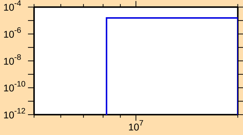
\sigma vs. E for ^{89}\text{Ru}(n,n\alpha)
