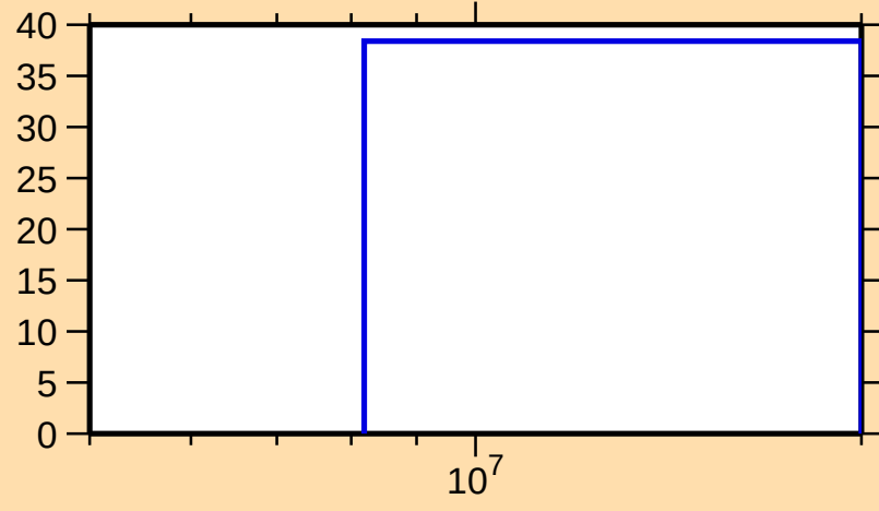
\Delta\sigma/\sigma vs. E for ^{89}\text{Ru}(n,2n)
