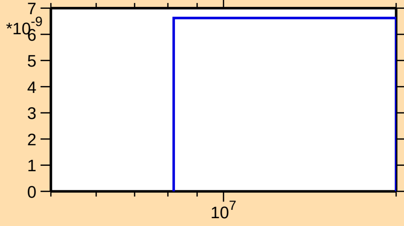
\sigma vs. E for ^{89}\text{Ru}(n,2np)
