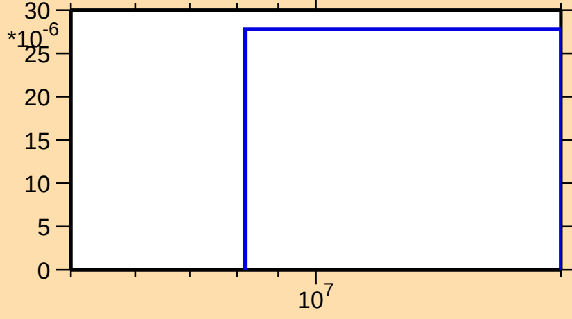
\sigma vs. E for ^{89}\text{Ru}(n,t)
