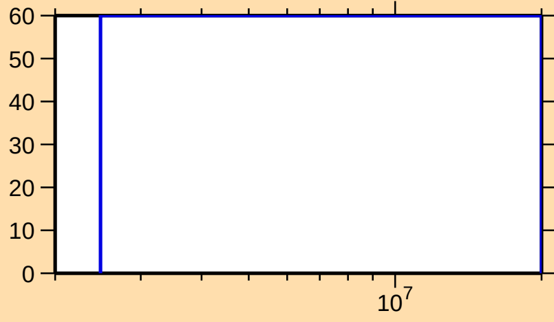
\Delta\sigma/\sigma vs. E for ^{89}\text{Ru}(n,n\text{cont.})
