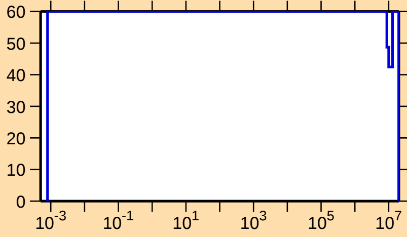
\Delta\sigma/\sigma vs. E for ^{90}\text{Ru}(n,\gamma)
