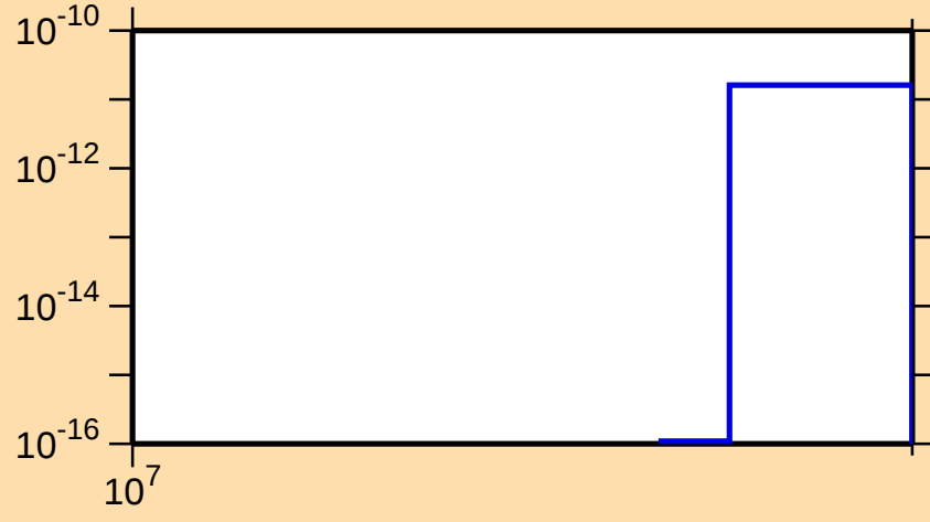
\sigma vs. E for ^{90}\text{Ru}(n,\text{nd})
