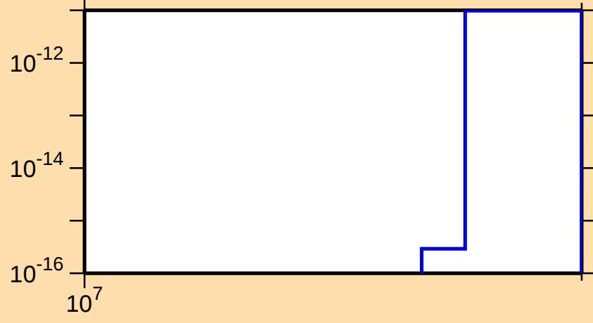
\sigma vs. E for ^{90}\text{Ru} (mt 34)
