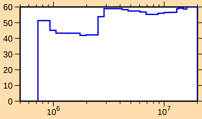
\Delta\sigma/\sigma vs. E for ^{90}\text{Ru}(n,n_1)
