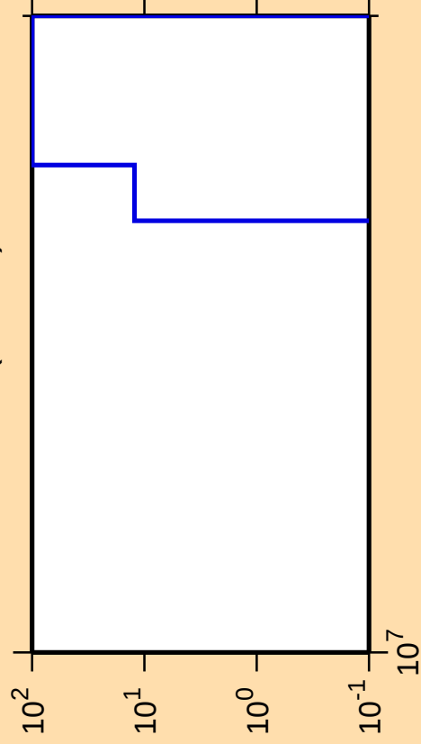
\Delta\sigma/\sigma vs. E for ^{90}\text{Ru}(\text{mt117})
