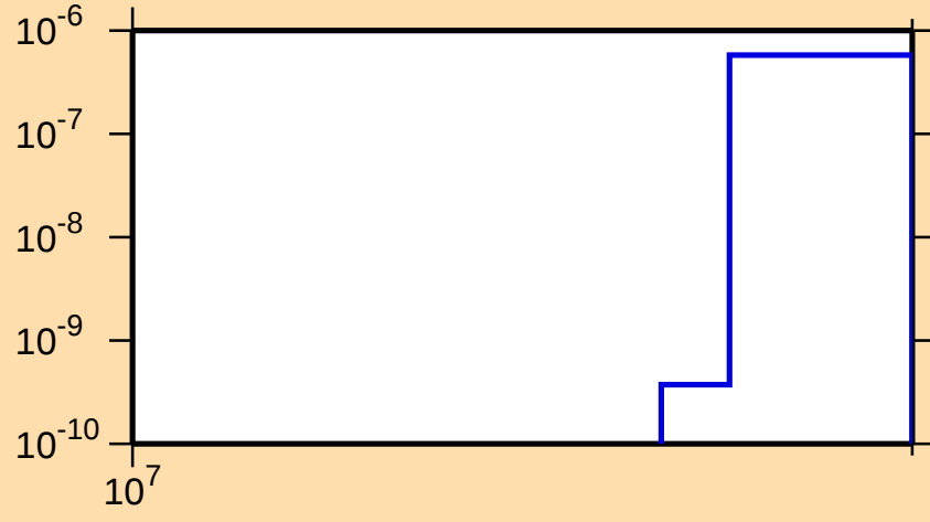
\sigma vs. E for ^{90}\text{Ru}(n,\text{pt})
