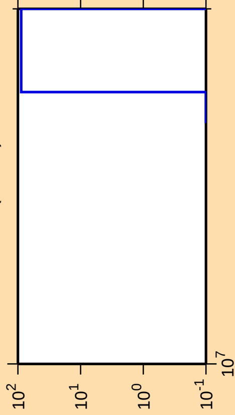
\Delta\sigma/\sigma vs. E for ^{90}\text{Ru} (mt 34)
