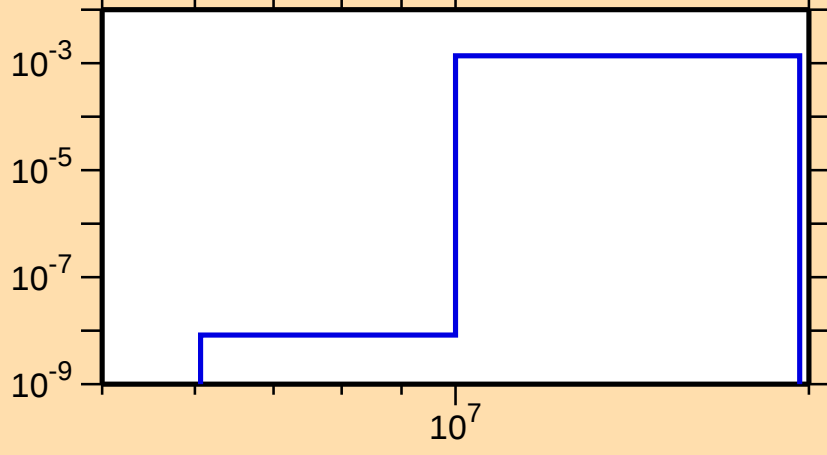
\sigma vs. E for ^{90}\text{Ru}(n,\text{pd})
