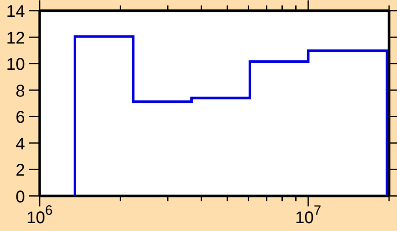
\Delta\sigma/\sigma vs. E for ^{90}\text{Ru}(n,n\text{nonel.})
