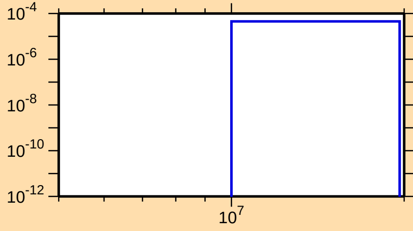
\sigma vs. E for ^{93}\text{Ru}(n,t)
