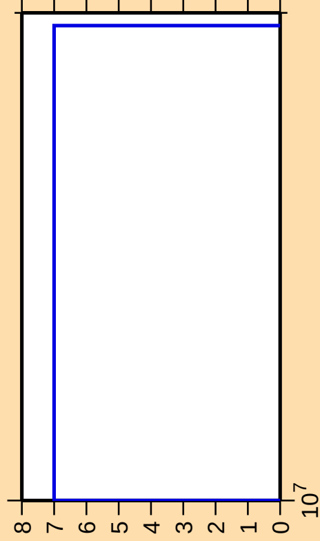
\Delta\sigma/\sigma vs. E for ^{93}\text{Ru}(\text{mt } 45)
