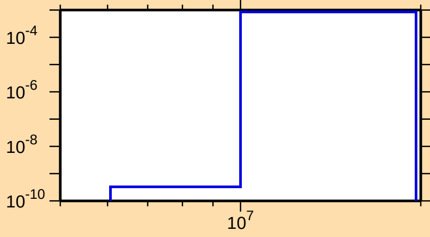
\sigma vs. E for ^{93}\text{Ru}(n,n\alpha)
