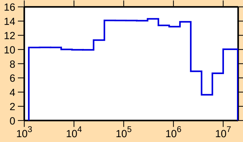
\Delta\sigma/\sigma vs. E for ^{93}\text{Ru}(\text{n,el.})
