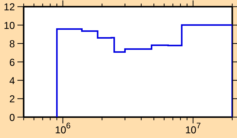
\Delta\sigma/\sigma vs. E for ^{93}\text{Ru}(n,n\text{nonel.})
