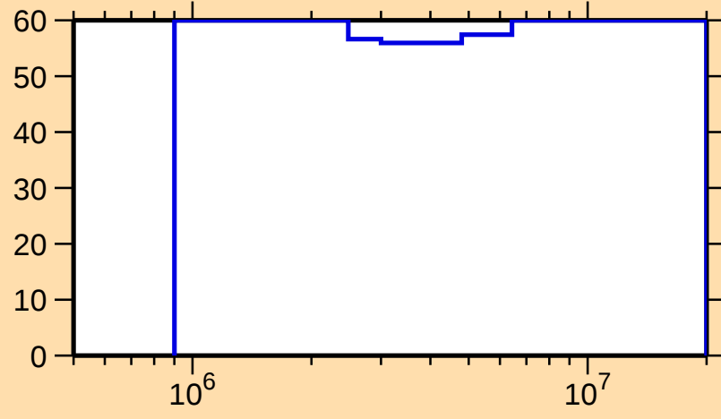
\Delta\sigma/\sigma vs. E for ^{93}\text{Ru}(n,ncont.)
