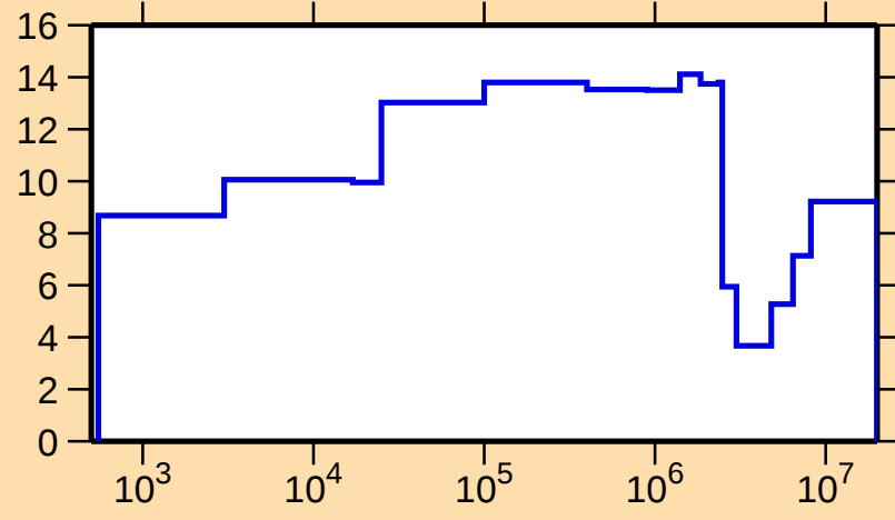
\Delta\sigma/\sigma vs. E for ^{93}\text{Ru}(\text{n,el.})
