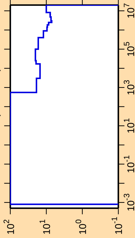
\Delta\sigma/\sigma vs. E for ^{93}\text{Ru}(n,\text{nonel.})
