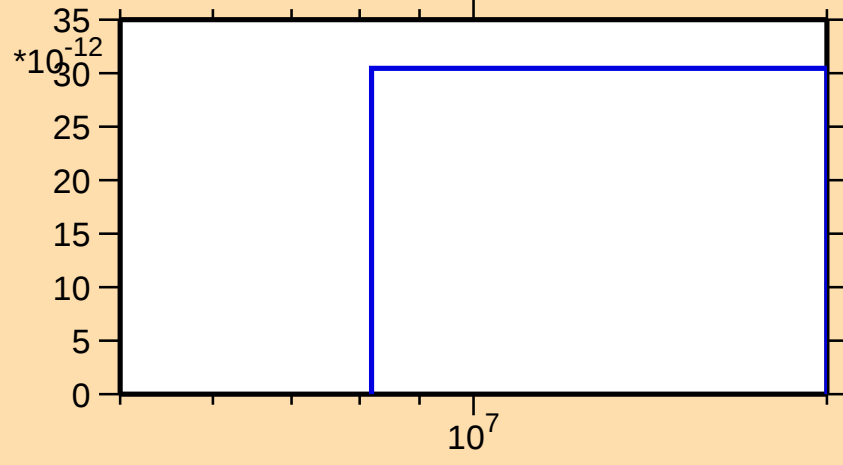
\sigma vs. E for ^{93}\text{Ru}(\text{mt } 34)
