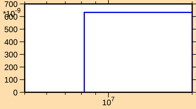
\sigma vs. E for ^{93}\text{Ru}(n,2np)
