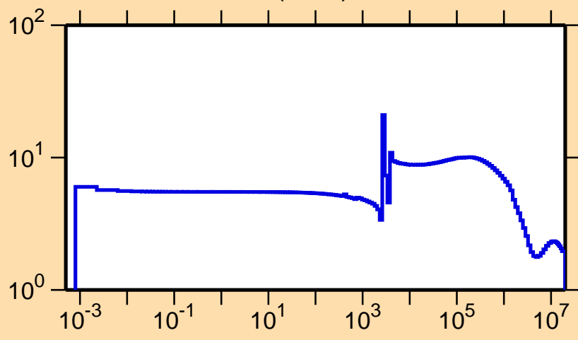
\sigma vs. E for ^{94}\text{Ru}(n,\text{el.})
