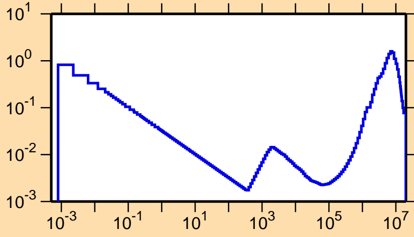
\sigma vs. E for ^{94}\text{Ru}(n,p)
