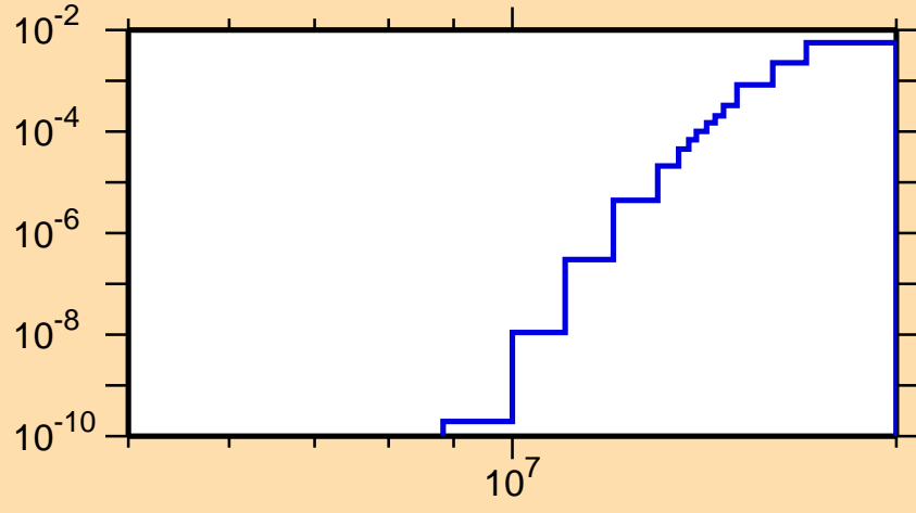
\sigma vs. E for ^{94}\text{Ru}(n,n\alpha)
