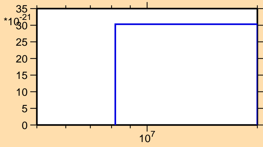
\sigma vs. E for ^{94}\text{Ru}(n,2n\alpha)
