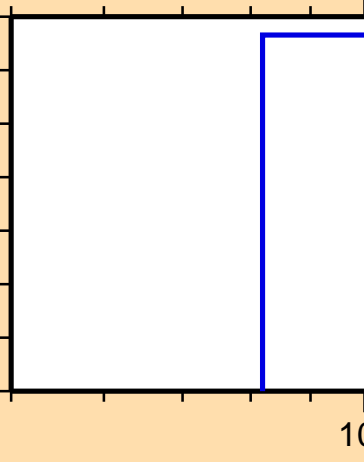
\sigma vs. E for ^{94}\text{Ru}(n,2np)
