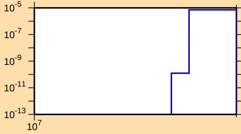
\sigma vs. E for ^{99}\text{Ru}(n,2np)
