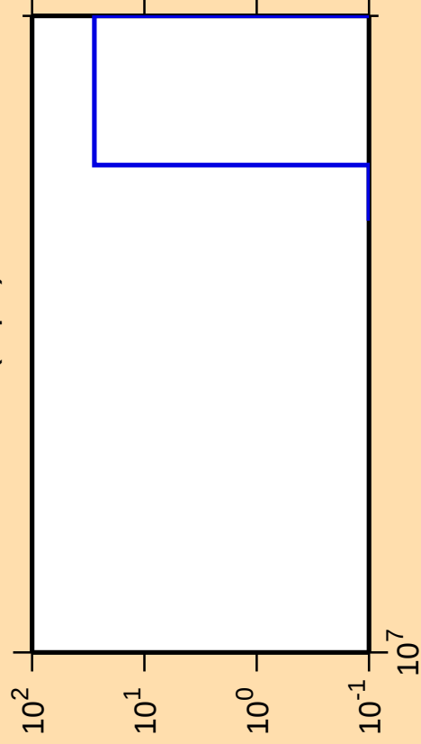
\Delta\sigma/\sigma vs. E for ^{99}\text{Ru}(n,\text{pd})
