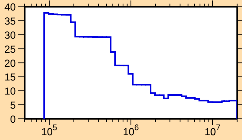
\Delta\sigma/\sigma vs. E for ^{99}\text{Ru}(\text{n,nonel.})
