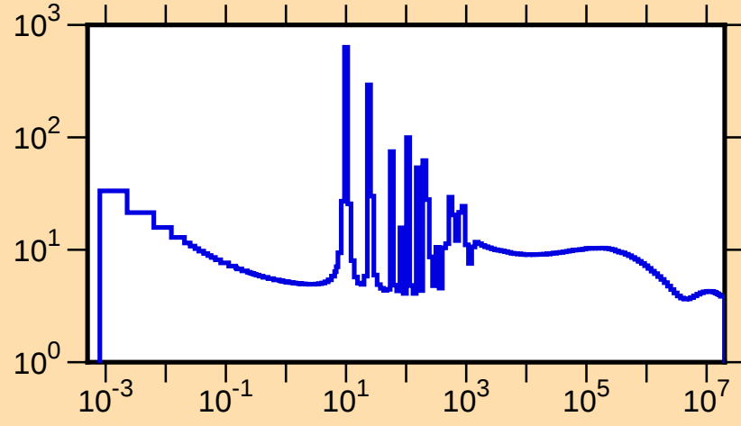
\sigma vs. E for ^{99}\text{Ru}(n,\text{tot.})
