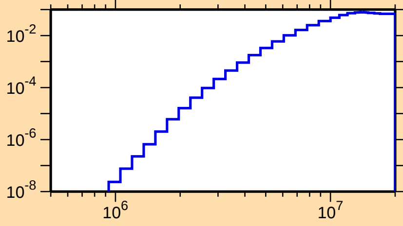
\sigma vs. E for ^{99}\text{Ru}(n,p)
