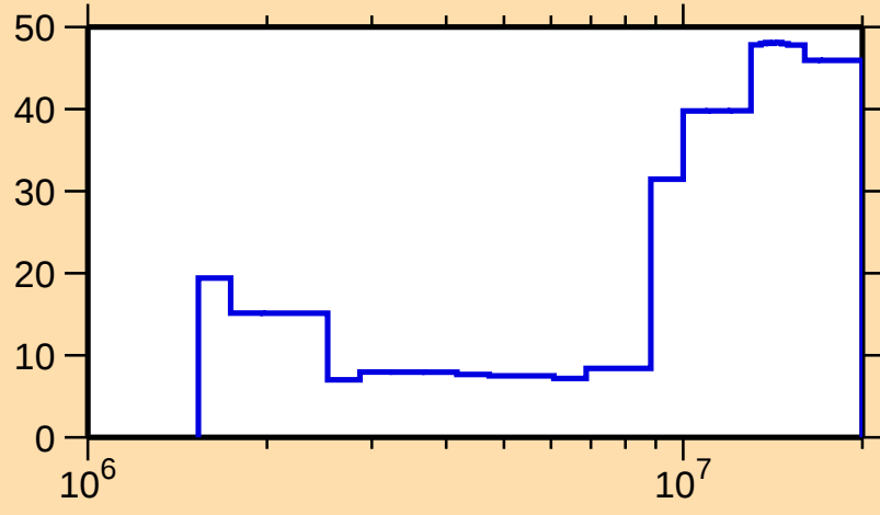
\Delta\sigma/\sigma vs. E for ^{99}\text{Ru}(n,n\text{cont.})
