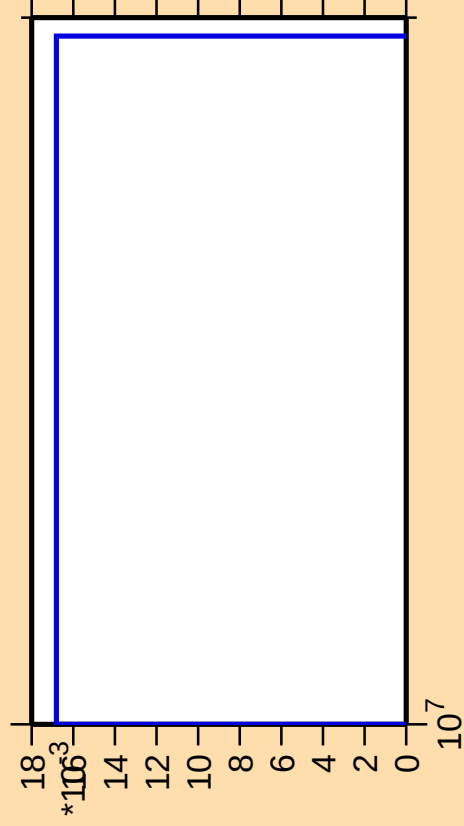
\Delta\sigma/\sigma vs. E for ^{99}\text{Ru}(\text{mt } 34)
