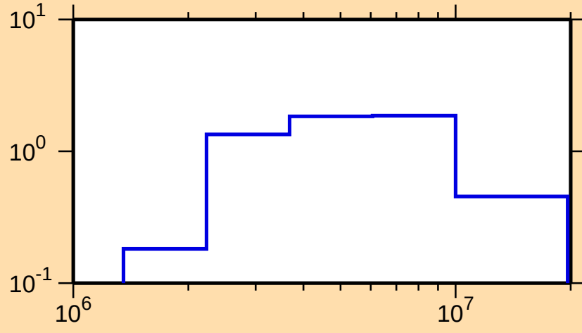
\sigma vs. E for ^{99}\text{Ru}(n,n\text{cont.})
