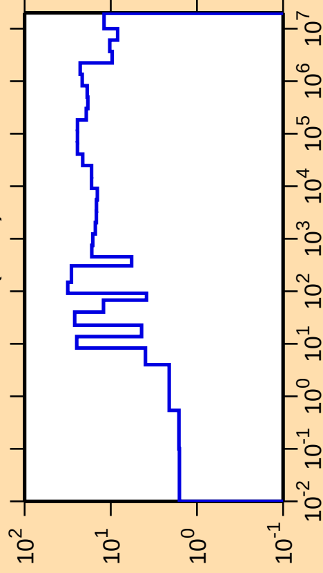
\Delta\sigma/\sigma vs. E for ^{99}\text{Ru}(n,\text{el.})
