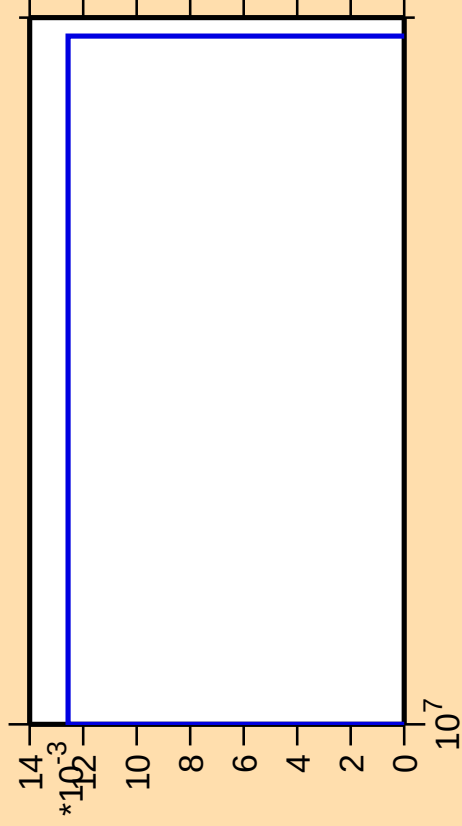
\Delta\sigma/\sigma vs. E for ^{99}\text{Ru}(\text{mt117})
