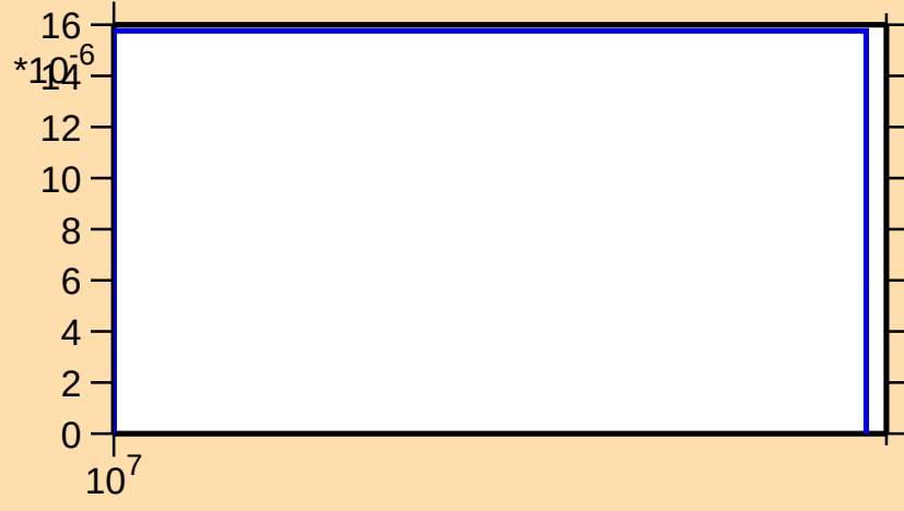
\sigma vs. E for ^{99}\text{Ru}(n,3n)
