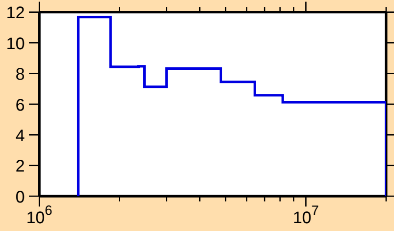
\Delta\sigma/\sigma vs. E for ^{99}\text{Ru}(\text{n},\text{nonel.})
