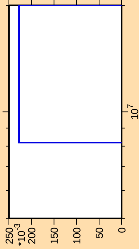
\Delta\sigma/\sigma vs. E for ^{99}\text{Ru}(n,\text{pd})
