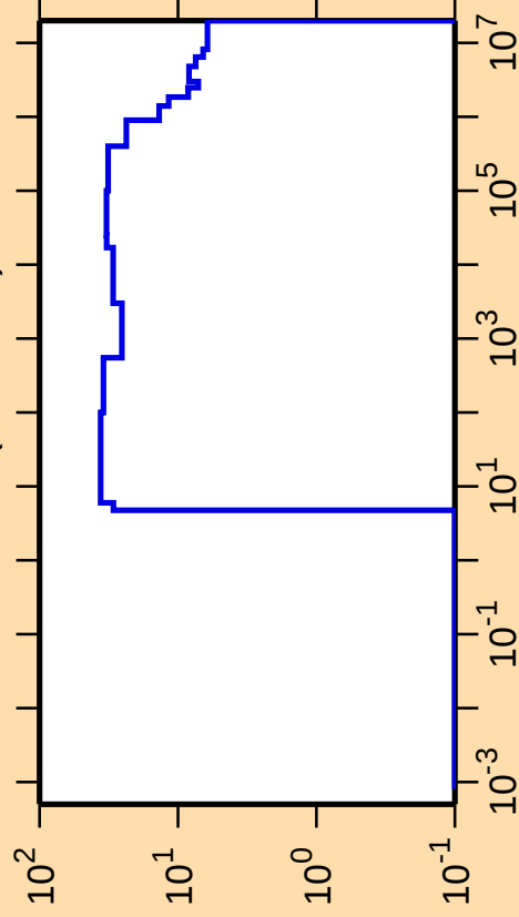
\Delta\sigma/\sigma vs. E for ^{99}\text{Ru}(n,\text{nonel.})
