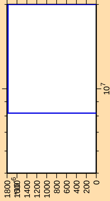
\Delta\sigma/\sigma vs. E for ^{99}\text{Ru}(\text{mt } 45)
