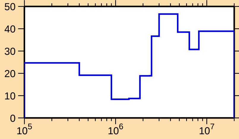
\Delta\sigma/\sigma vs. E for ^{99}\text{Ru}(n,n_1)
