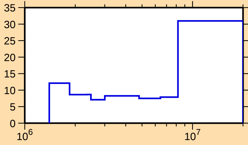
\Delta\sigma/\sigma vs. E for ^{99}\text{Ru}(n,\text{inel.})
