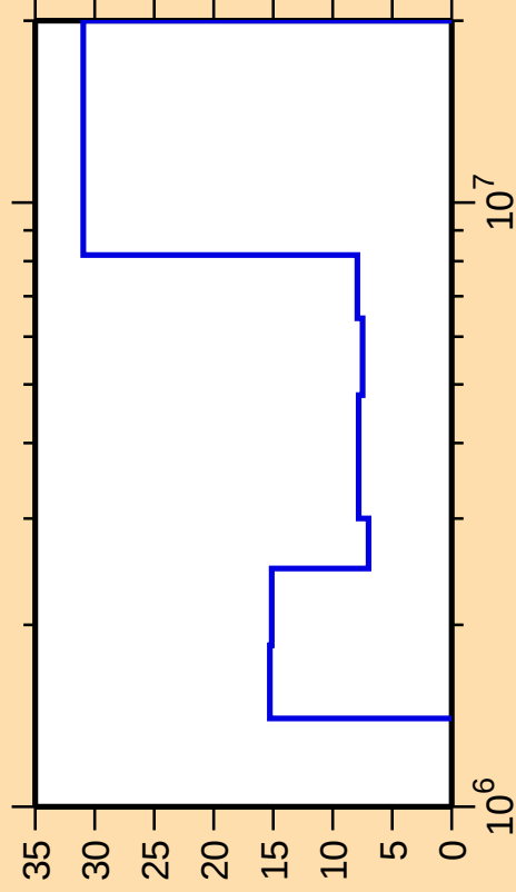
\Delta\sigma/\sigma vs. E for ^{99}\text{Ru}(\text{n},\text{ncont.})
