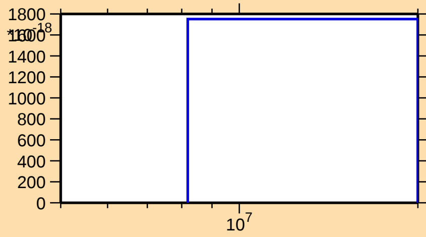
\sigma vs. E for ^{99}\text{Ru}(\text{mt } 45)
