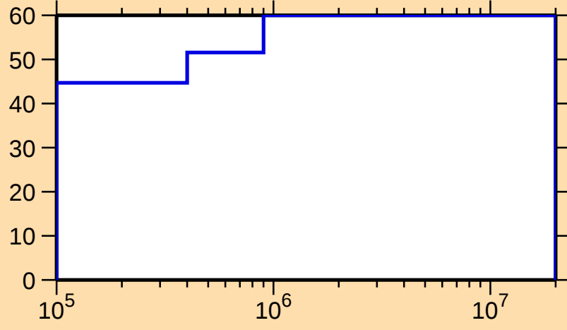
\Delta\sigma/\sigma vs. E for ^{99}\text{Ru}(n,\gamma)
