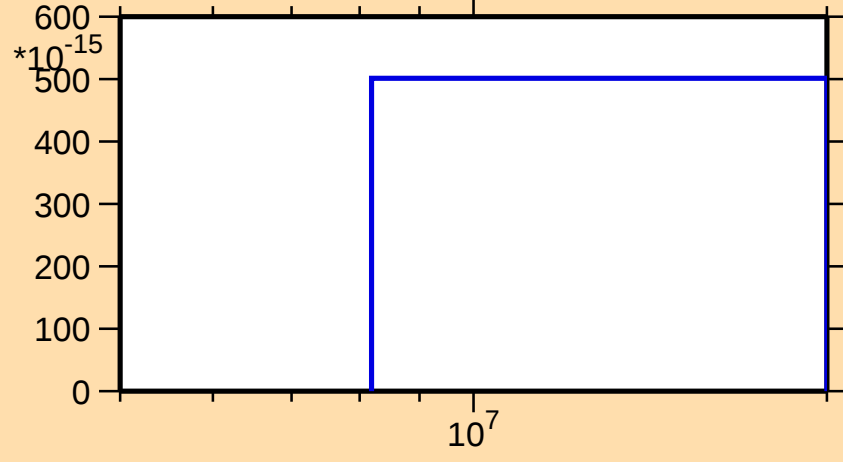
\sigma vs. E for ^{99}\text{Ru}(n,\text{pt})
