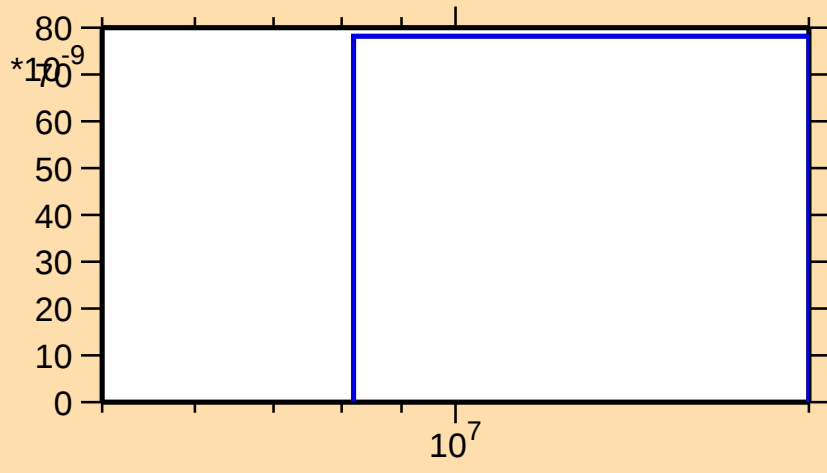
\sigma vs. E for ^{99}\text{Ru}(n,\text{He}3)
