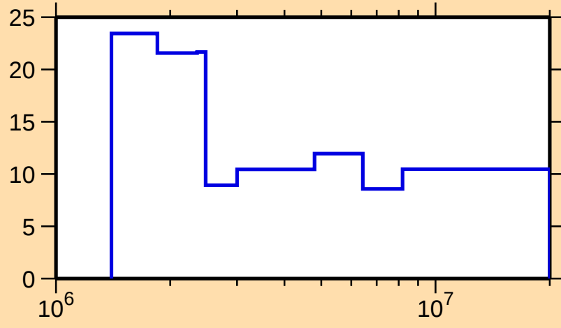
\Delta\sigma/\sigma vs. E for ^{99}\text{Ru}(n,\text{el.})
