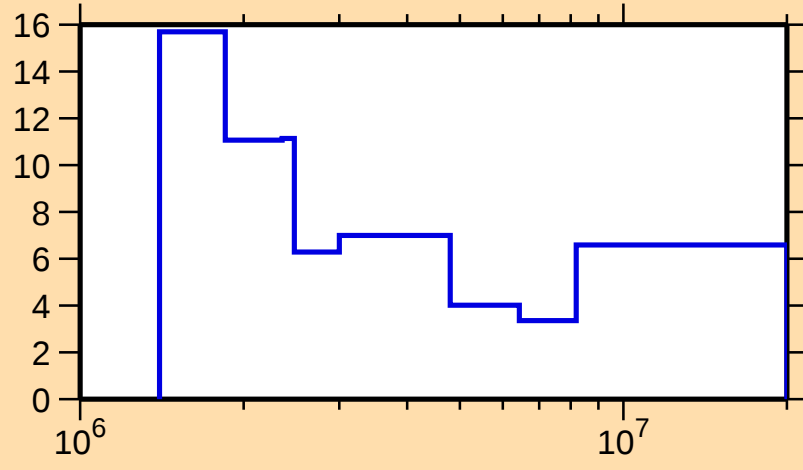
\Delta\sigma/\sigma vs. E for ^{99}\text{Ru}(n,\text{tot.})
