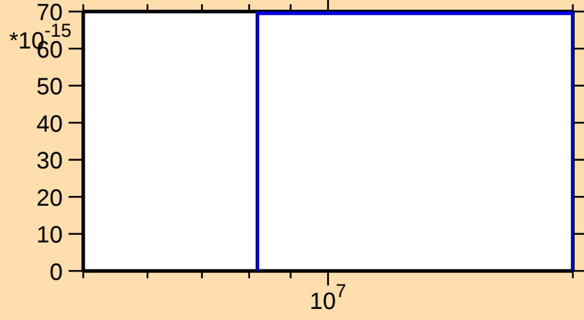
\sigma vs. E for ^{99}\text{Ru}(n,\text{pd})
