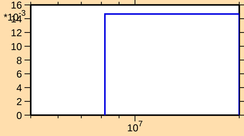
\sigma vs. E for ^{99}\text{Ru}(n,np)
