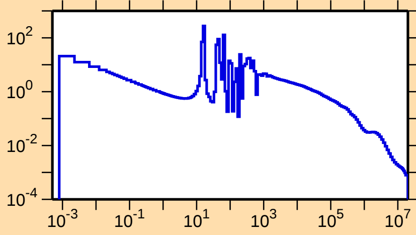
\sigma vs. E for ^{101}\text{Ru}(n,\gamma)
