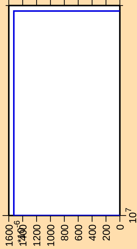
\Delta\sigma/\sigma vs. E for ^{106}\text{Ru}(n,\text{He}3)
