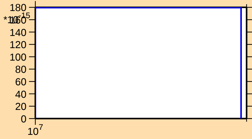
\sigma vs. E for ^{106}\text{Ru}(n,nt)
