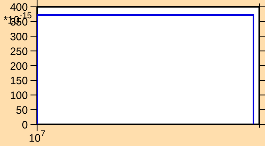
\sigma vs. E for ^{106}\text{Ru}(n,\text{nd})
