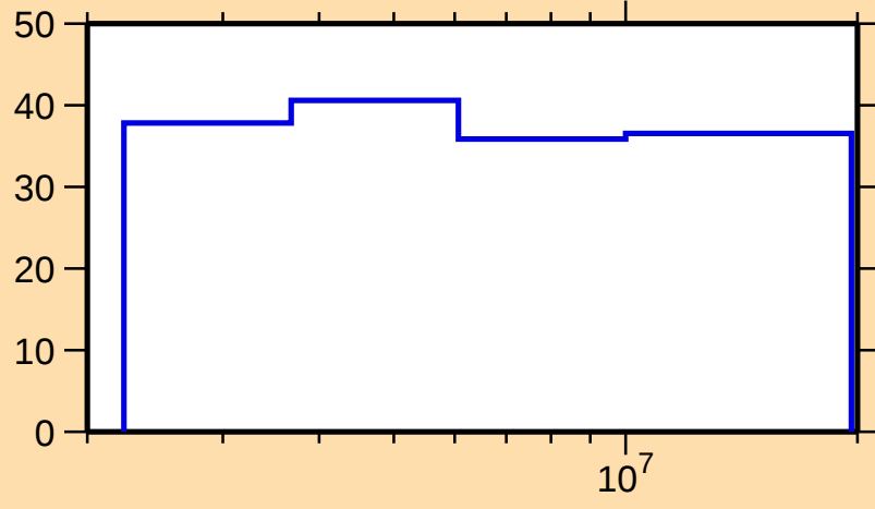
\Delta\sigma/\sigma vs. E for ^{106}\text{Ru}(n,n_1)
