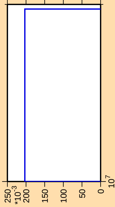
\Delta\sigma/\sigma vs. E for ^{106}\text{Ru}(n,2n\alpha)
