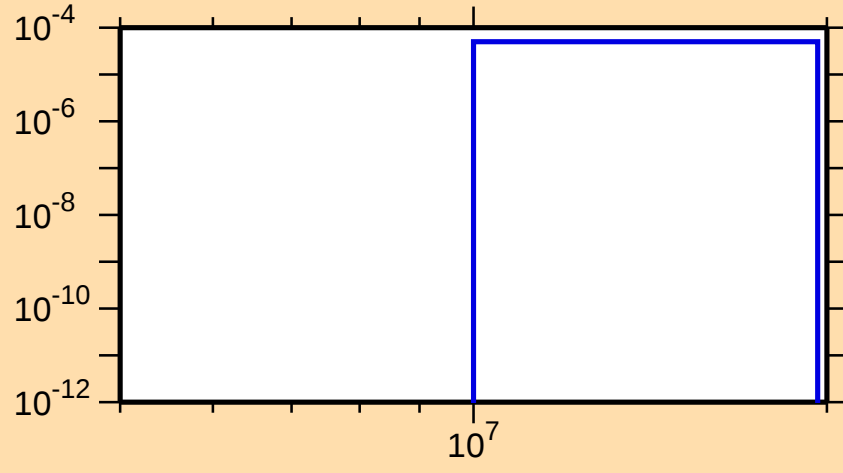
\sigma vs. E for ^{106}\text{Ru}(n,d)
