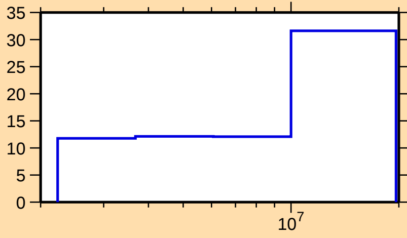
\Delta\sigma/\sigma vs. E for ^{106}\text{Ru}(n,\text{inel.})
