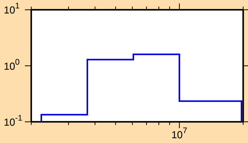
\sigma vs. E for ^{106}\text{Ru}(n,n\text{cont.})
