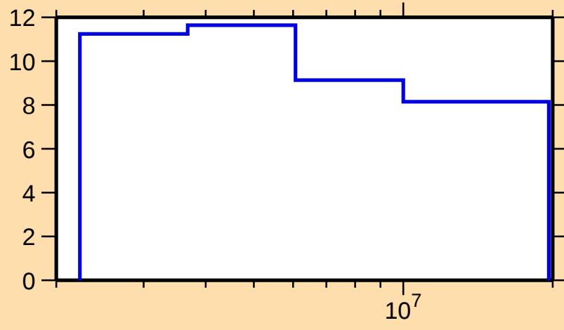
\Delta\sigma/\sigma vs. E for ^{106}\text{Ru}(n,n\text{onel.})
