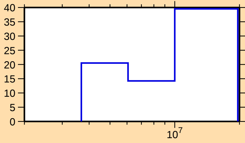
\Delta\sigma/\sigma vs. E for ^{106}\text{Ru}(n,n\text{cont.})
