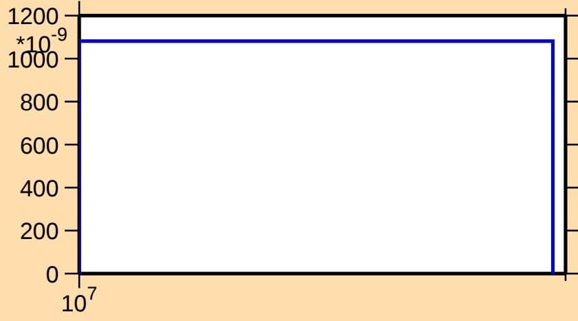
\sigma vs. E for ^{106}\text{Ru}(n,t)
