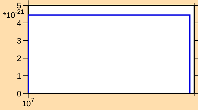
\sigma vs. E for ^{106}\text{Ru}(n,2np)
