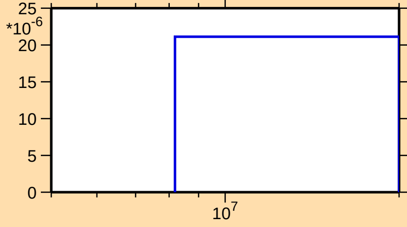
\sigma vs. E for ^{106}\text{Ru}(n,np)
