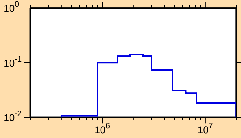
\sigma vs. E for ^{106}\text{Ru}(n,n_2)
