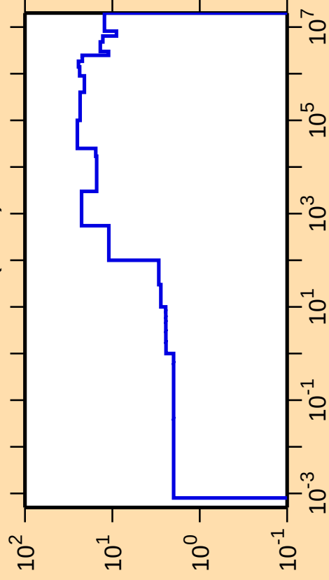
\Delta\sigma/\sigma vs. E for ^{106}\text{Ru}(n,\text{el.})
