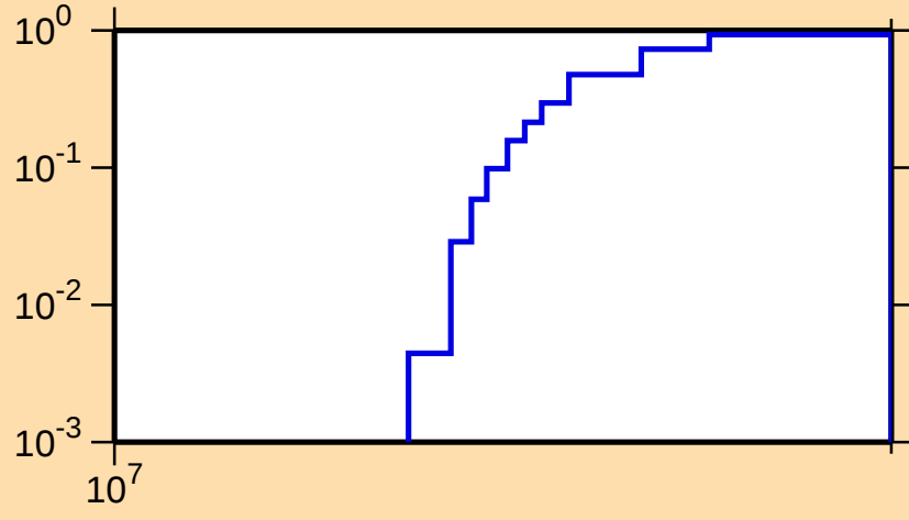
\sigma vs. E for ^{109}\text{Ru}(n,3n)
