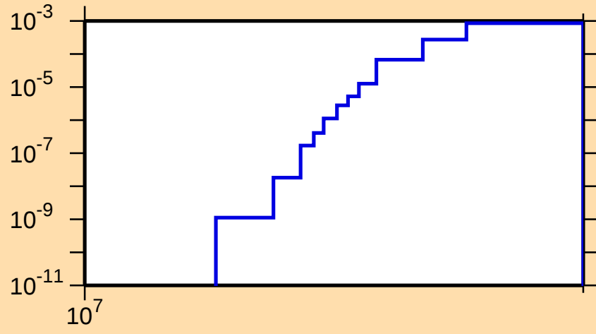
\sigma vs. E for ^{109}\text{Ru}(n,d)
