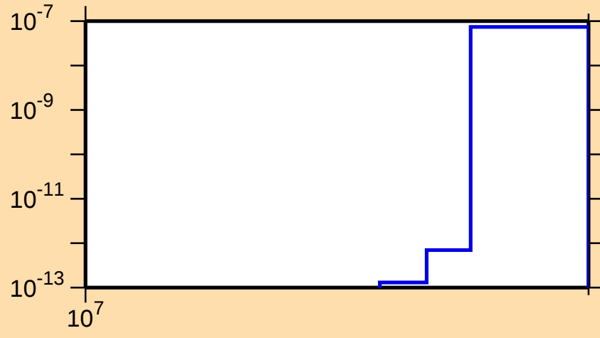
\sigma vs. E for ^{109}\text{Ru}(n,\text{nd})
