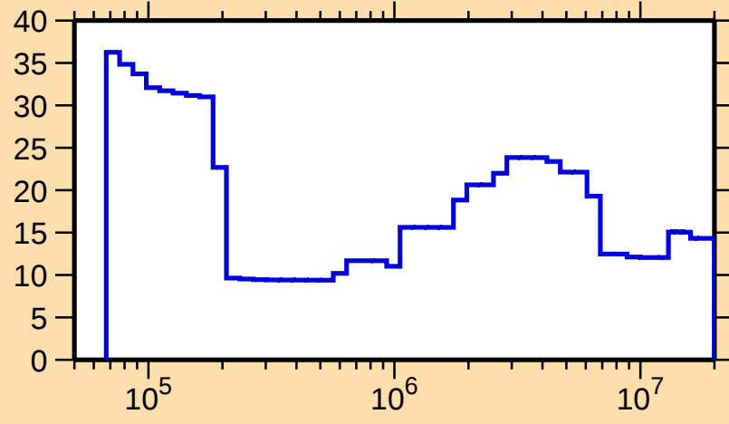
\Delta\sigma/\sigma vs. E for ^{109}\text{Ru}(\text{n,nonel.})
