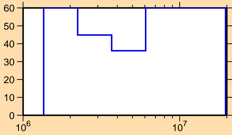
\Delta\sigma/\sigma vs. E for ^{109}\text{Ru}(n,n\text{cont.})
