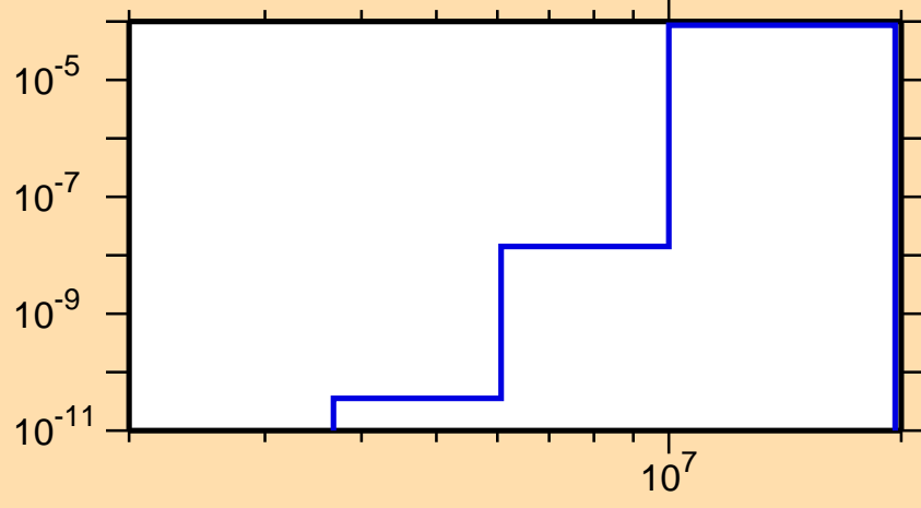
\sigma vs. E for ^{109}\text{Ru}(n,\alpha)
