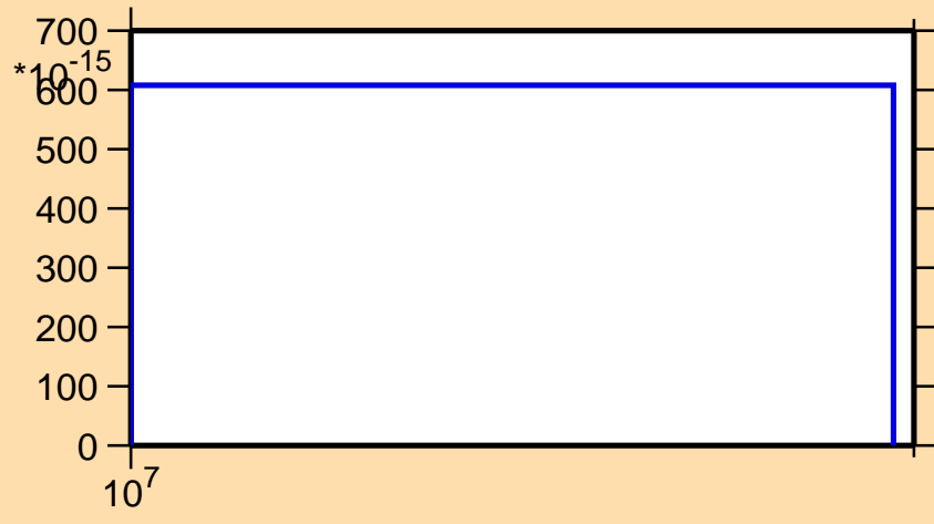
\sigma vs. E for ^{109}\text{Ru}(n,2np)
