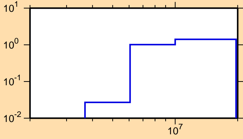
\sigma vs. E for ^{109}\text{Ru}(n,2n)
