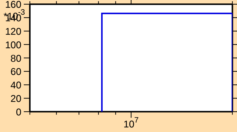
\sigma vs. E for ^{109}\text{Ru}(n,3n)
