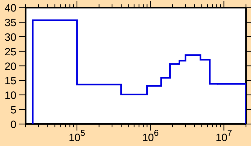
\Delta\sigma/\sigma vs. E for ^{109}\text{Ru}(n,\text{nonel.})
