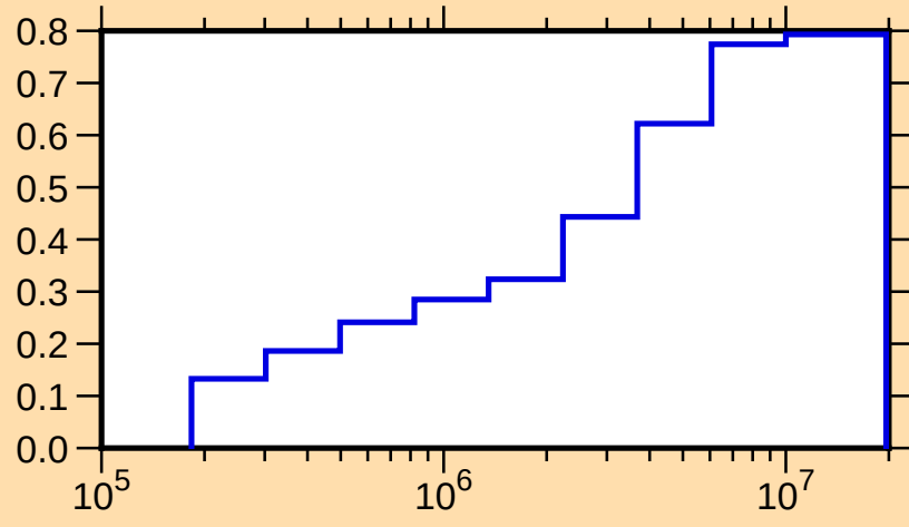
\mu vs. E for ^{32}\text{S}(\text{mt251})
