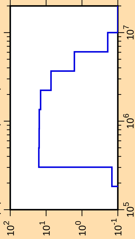
\Delta\mu/\mu vs. E for ^{32}\text{S}(\text{mt251})
