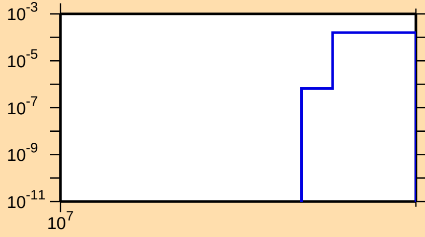
\sigma vs. E for ^{33}\text{S}(\text{n},\text{nd})
