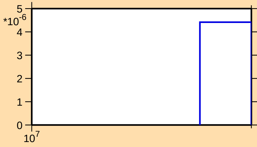
\sigma vs. E for ^{33}\text{S}(\text{n},2\text{np})
