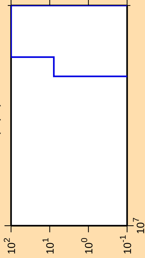
\Delta\sigma/\sigma vs. E for ^{33}\text{S}(\text{n},\text{pd})
