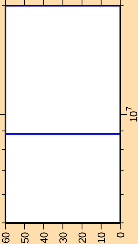
\Delta\sigma/\sigma vs. E for ^{33}\text{S}(n,\gamma)
