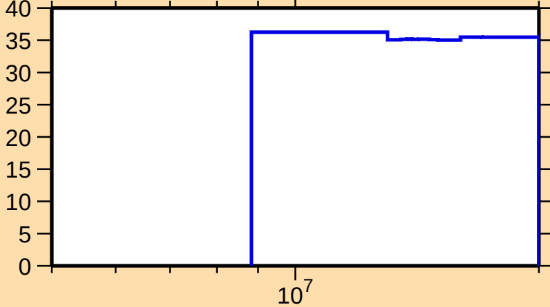
\Delta\sigma/\sigma vs. E for ^{33}\text{S}(n,2n)
