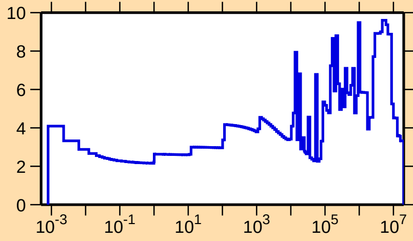
\Delta\sigma/\sigma vs. E for ^{33}\text{S}(\text{n,tot.})
