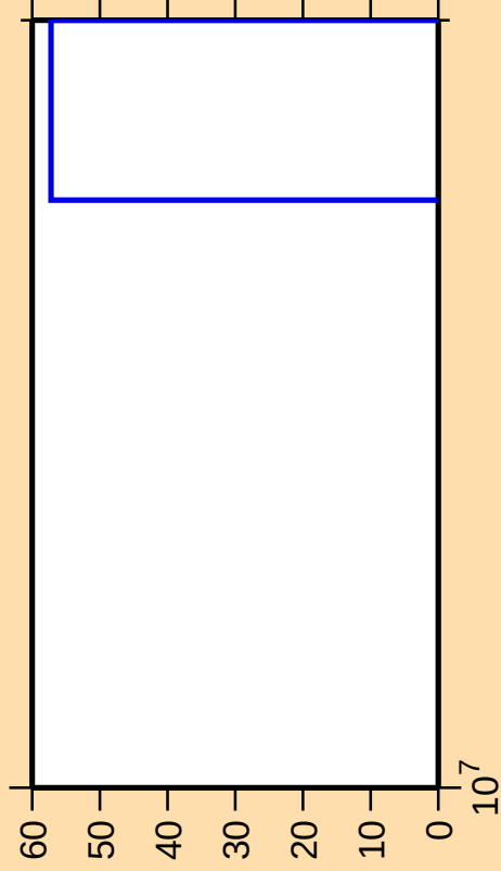
\Delta\sigma/\sigma vs. E for ^{33}\text{S}(\text{n},2\text{np})
