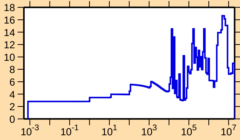
\Delta\sigma/\sigma vs. E for ^{33}\text{S}(\text{n,el.})
