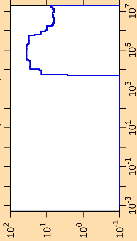
\Delta\sigma/\sigma vs. E for ^{33}\text{S}(\text{n,nonel.})
