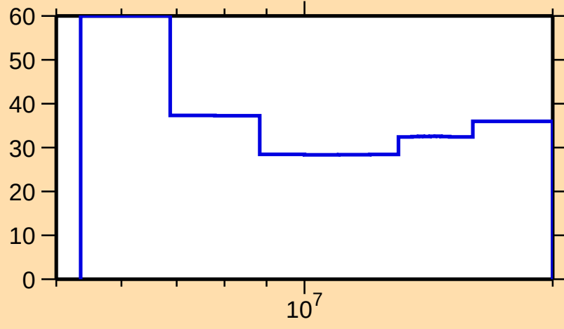
\Delta\sigma/\sigma vs. E for ^{33}\text{S}(n,\text{ncont.})
