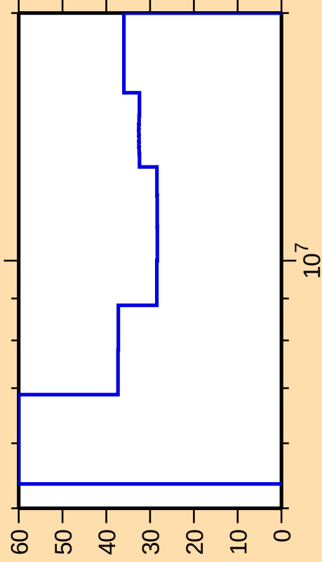
\Delta\sigma/\sigma vs. E for ^{33}\text{S}(\text{n},\text{ncont.})
