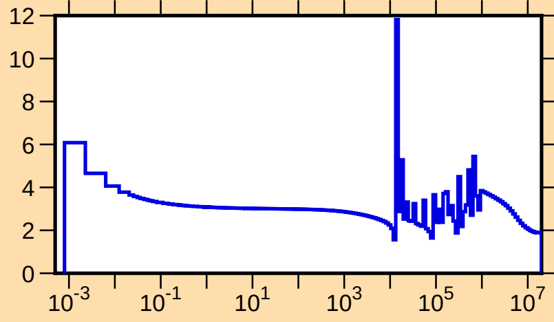
\sigma vs. E for ^{33}\text{S}(\text{n,tot.})
