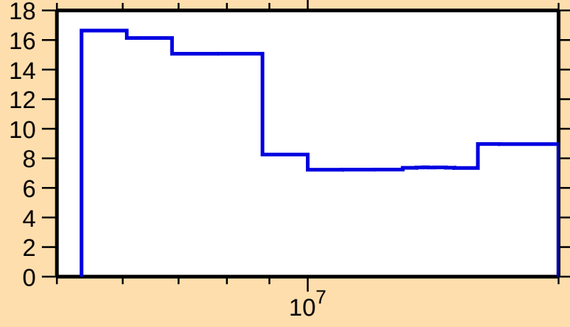
\Delta\sigma/\sigma vs. E for ^{33}\text{S}(\text{n},\text{el.})
