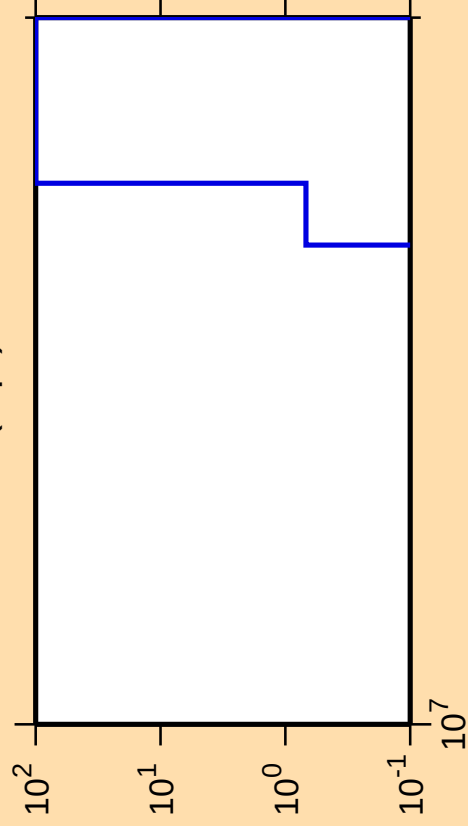
\Delta\sigma/\sigma vs. E for ^{33}\text{S}(\text{n},\text{pt})
