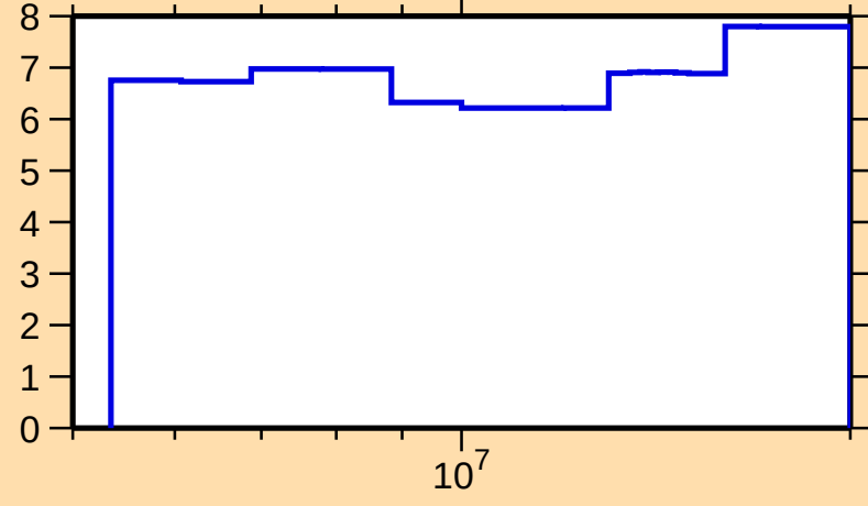
\Delta\sigma/\sigma vs. E for ^{33}\text{S}(\text{n},\text{nonel.})
