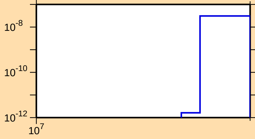
\sigma vs. E for ^{33}\text{S}(\text{n},\text{pd})
