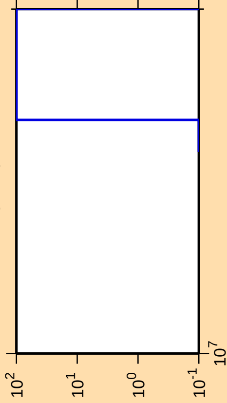
\Delta\sigma/\sigma vs. E for ^{33}\text{S}(\text{n},\text{nd})
