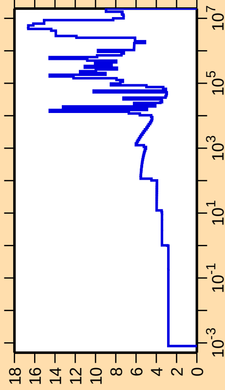
\Delta\sigma/\sigma vs. E for ^{33}\text{S}(\text{n,el.})
