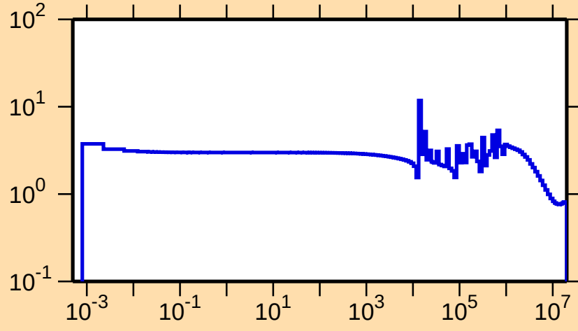
\sigma vs. E for ^{33}\text{S}(\text{n,el.})
