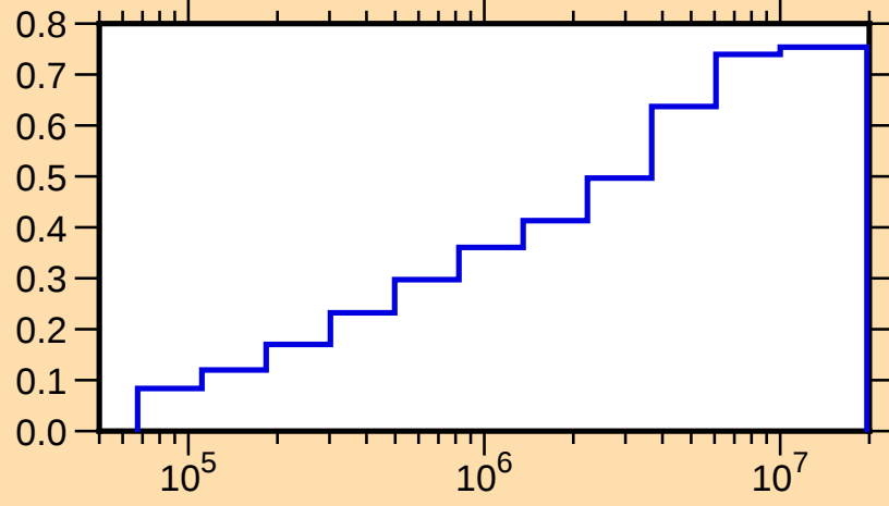
\mu vs. E for ^{33}\text{S}(\text{mt251})
