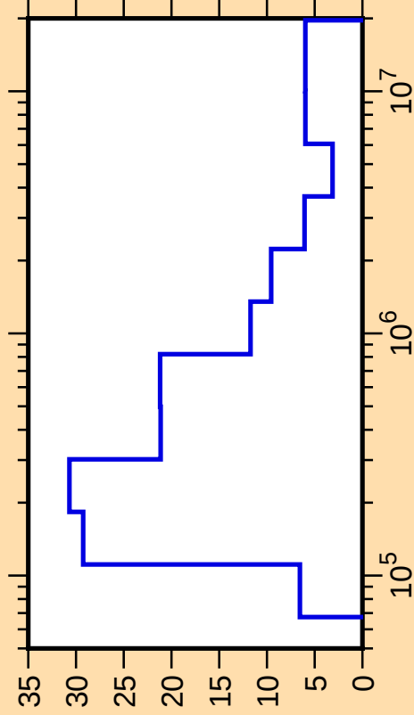
\Delta\mu/\mu vs. E for ^{33}\text{S}(\text{mt251})
