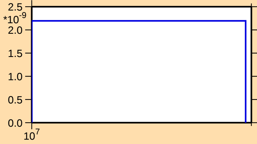
\sigma vs. E for ^{33}\text{S}(\text{n},\text{pt})
