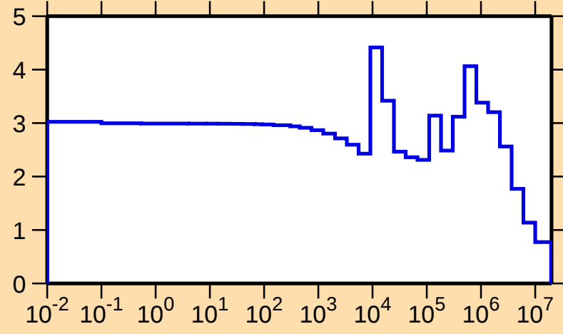
\sigma vs. E for ^{33}\text{S}(\text{n,el.})
