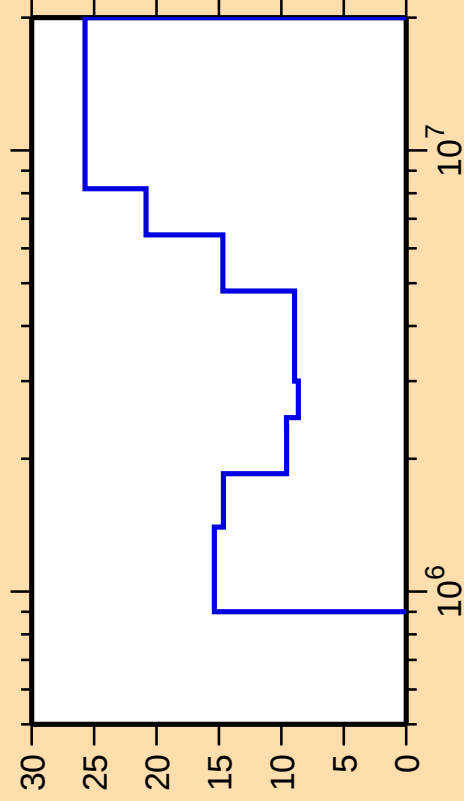
\Delta\sigma/\sigma vs. E for ^{33}\text{S}(\text{n,inel.})
