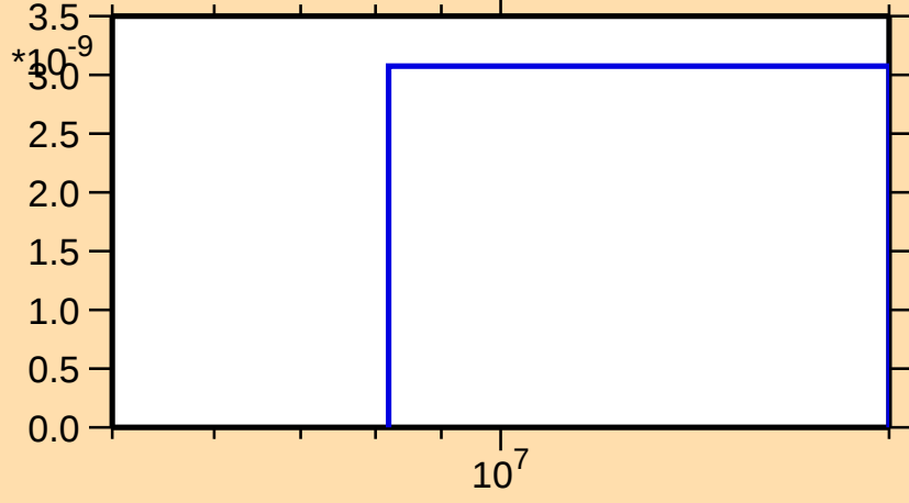
\sigma vs. E for ^{33}\text{S}(\text{n},\text{pt})
