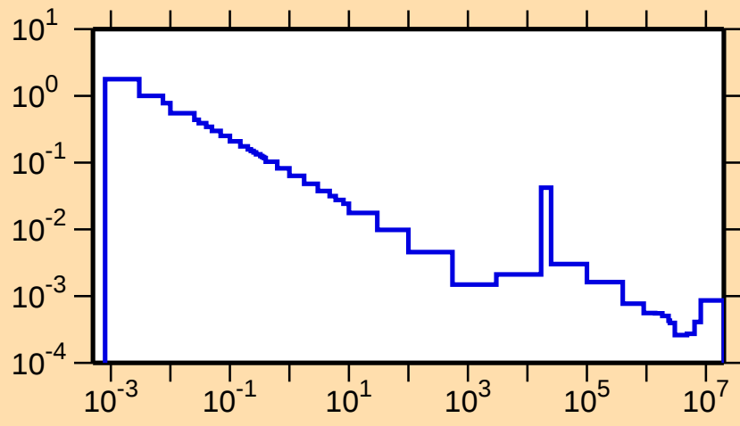
\sigma vs. E for ^{33}\text{S}(n,\gamma)
