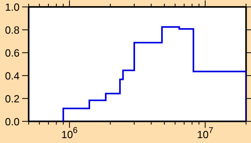
\sigma vs. E for ^{33}\text{S}(\text{n,inel.})
