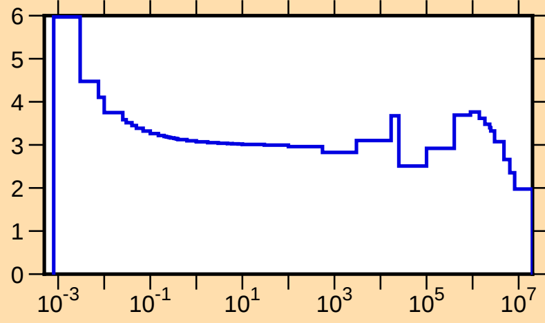
\sigma vs. E for ^{33}\text{S}(\text{n,tot.})
