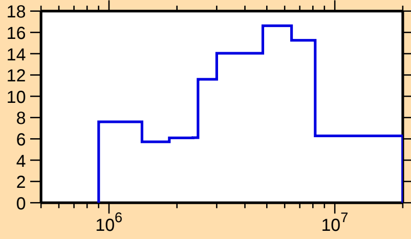
\Delta\sigma/\sigma vs. E for ^{33}\text{S}(\text{n,el.})
