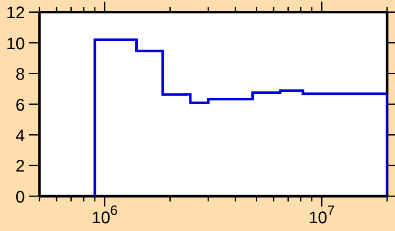
\Delta\sigma/\sigma vs. E for ^{33}\text{S}(\text{n,nonel.})
