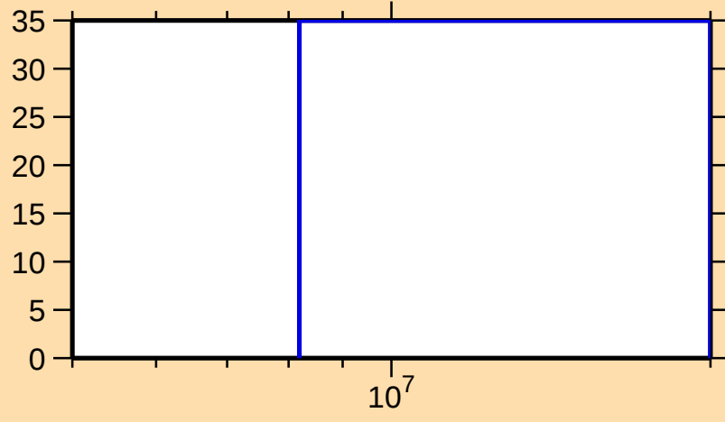
\Delta\sigma/\sigma vs. E for ^{33}\text{S}(\text{n},2\text{n})
