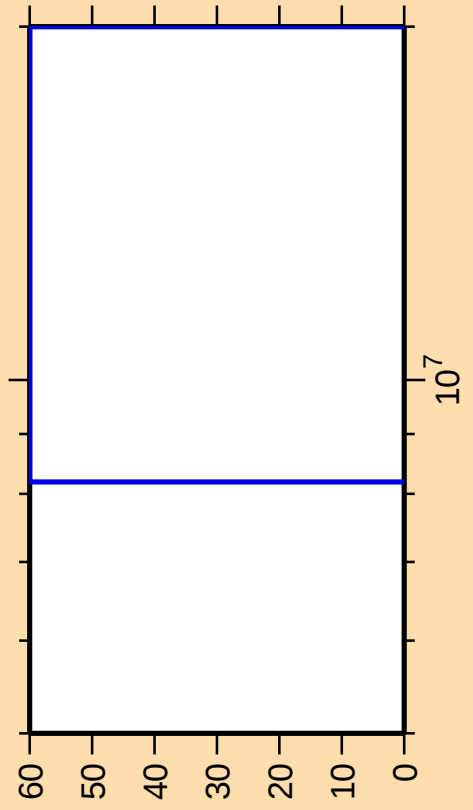
\Delta\sigma/\sigma vs. E for ^{33}\text{S}(n,\gamma)
