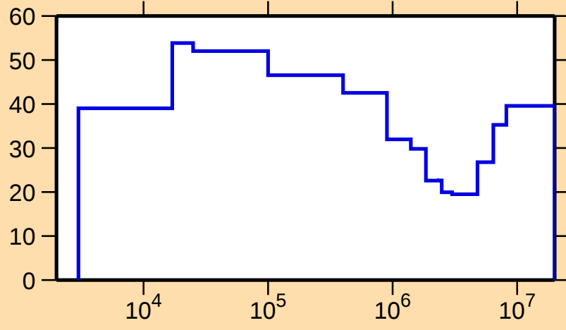
\Delta\sigma/\sigma vs. E for ^{33}\text{S}(n,p)
