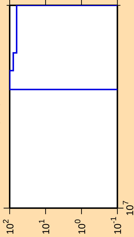
\Delta\sigma/\sigma vs. E for ^{40}\text{S}(\text{n,d})
