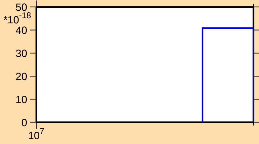
\sigma vs. E for ^{40}\text{S}(n,2n\alpha)
