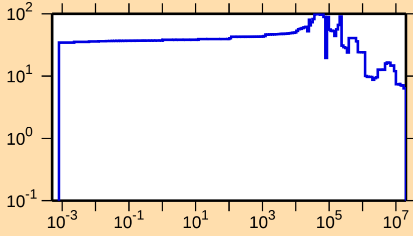
\Delta\sigma/\sigma vs. E for ^{40}\text{S}(\text{n,tot.})
