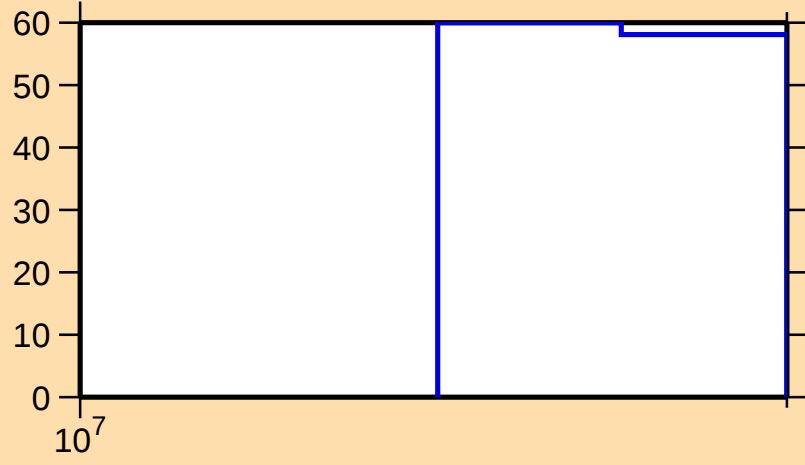
\Delta\sigma/\sigma vs. E for ^{40}\text{S}(\text{n,n}_1)
