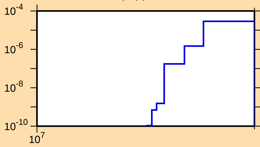
\sigma vs. E for ^{40}\text{S}(\text{n,p})
