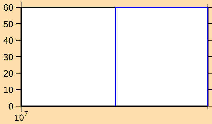
\Delta\sigma/\sigma vs. E for ^{40}\text{S}(\text{n,ncont.})
