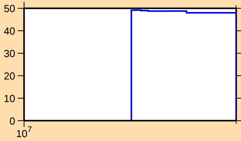
\Delta\sigma/\sigma vs. E for ^{40}\text{S}(\text{n,inel.})
