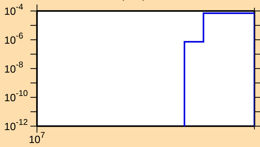
\sigma vs. E for ^{40}\text{S}(\text{n,d})
