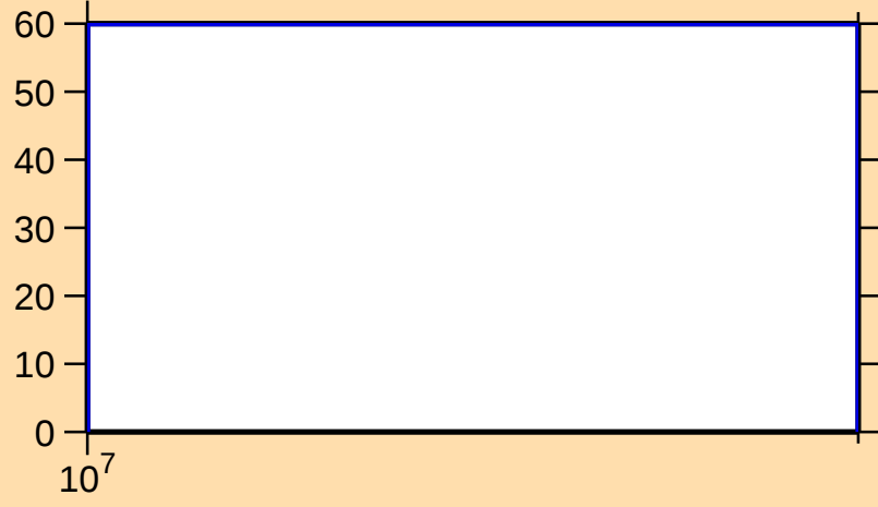
\Delta\sigma/\sigma vs. E for ^{40}\text{S}(n,\gamma)
