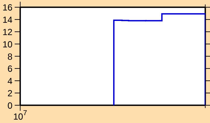
\Delta\sigma/\sigma vs. E for ^{40}\text{S}(\text{n,nonel.})
