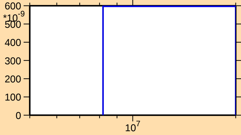
\sigma vs. E for ^{40}\text{S}(\text{n,d})
