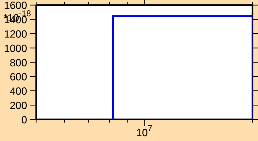
\sigma vs. E for ^{40}\text{S}(\text{n},\text{nt})
