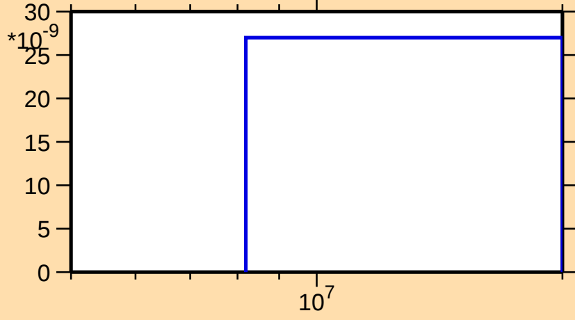
\sigma vs. E for ^{40}\text{S}(\text{n,t})
