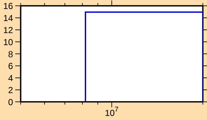
\Delta\sigma/\sigma vs. E for ^{40}\text{S}(\text{n,el.})
