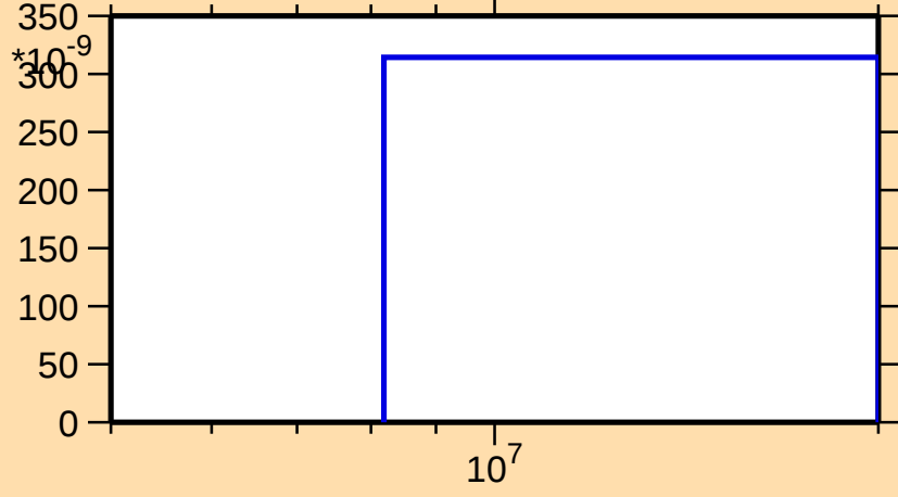
\sigma vs. E for ^{40}\text{S}(\text{n,p})
