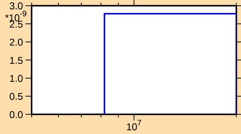
\sigma vs. E for ^{40}\text{S}(\text{n},\text{np})
