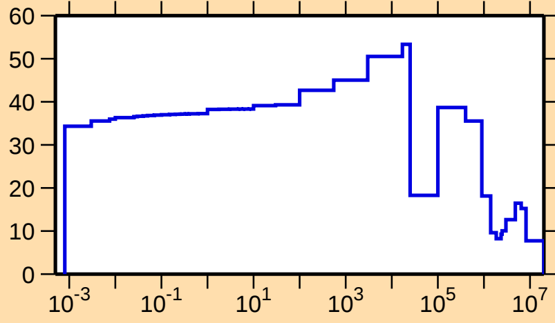
\Delta\sigma/\sigma vs. E for ^{40}\text{S}(\text{n,tot.})
