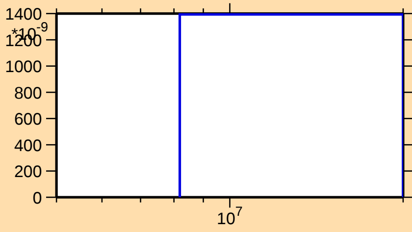
\sigma vs. E for ^{40}\text{S}(n,\alpha)
