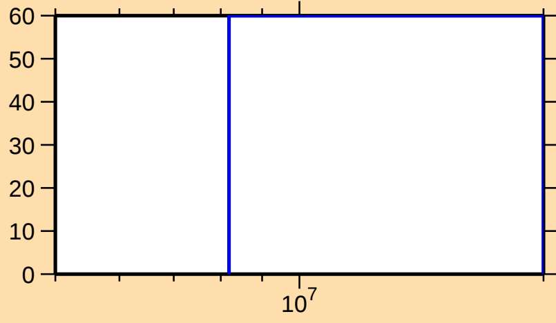
\Delta\sigma/\sigma vs. E for ^{40}\text{S}(\text{n,ncont.})
