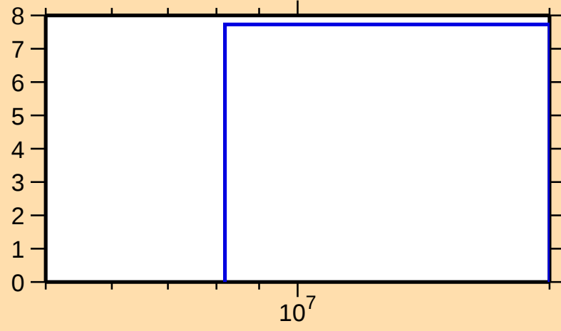
\Delta\sigma/\sigma vs. E for ^{40}\text{S}(\text{n,tot.})
