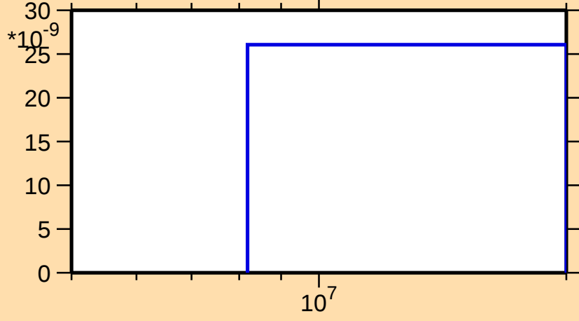
\sigma vs. E for ^{40}\text{S}(n,n\alpha)
