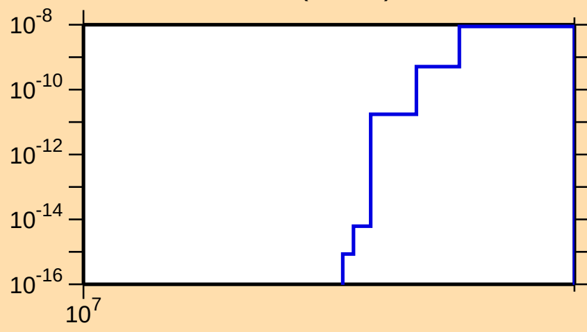
\sigma vs. E for ^{107}\text{Sb}(n,2n\alpha)
