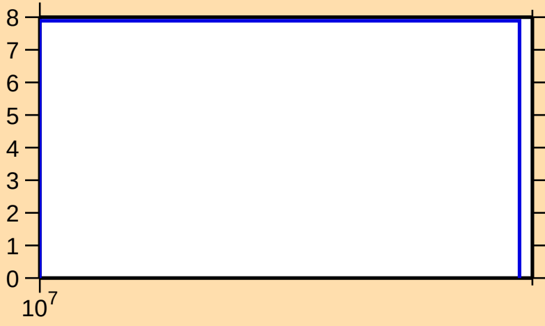
\Delta\sigma/\sigma vs. E for ^{107}\text{Sb}(n,\text{nonel.})
