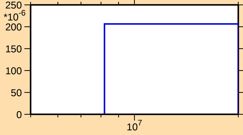
\sigma vs. E for ^{107}\text{Sb}(n,2n)
