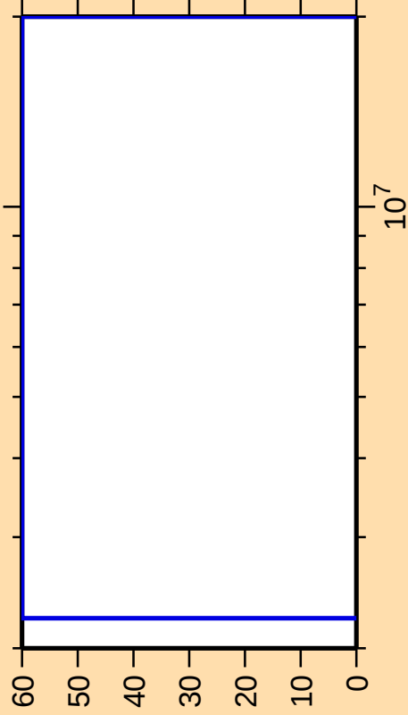
\Delta\sigma/\sigma vs. E for ^{111}\text{Sb}(n,\text{ncont.})
