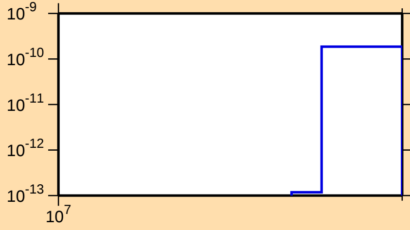
\sigma vs. E for ^{111}\text{Sb}(\text{mt } 34)
