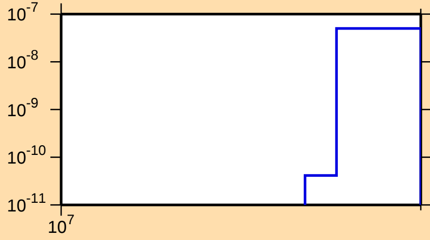
\sigma vs. E for ^{111}\text{Sb}(n,\text{pt})
