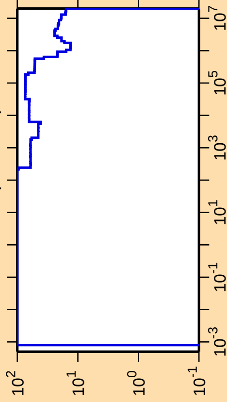
\Delta\sigma/\sigma vs. E for ^{111}\text{Sb}(n,\text{nonel.})
