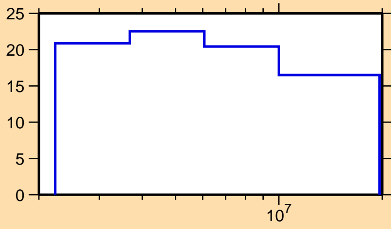
\Delta\sigma/\sigma vs. E for ^{111}\text{Sb}(n,n\text{onel.})
