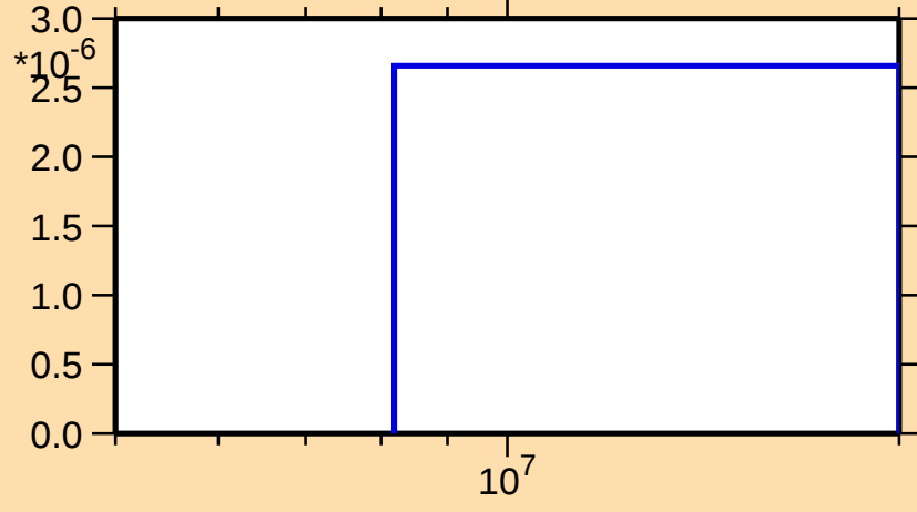
\sigma vs. E for ^{111}\text{Sb}(n,\text{pd})
