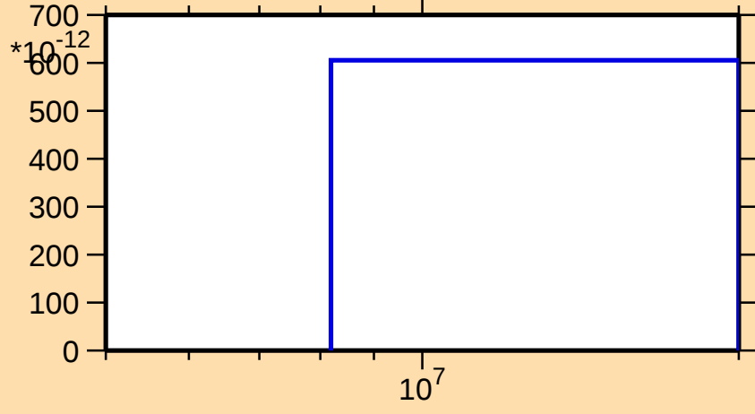
\sigma vs. E for ^{111}\text{Sb}(n,nt)
