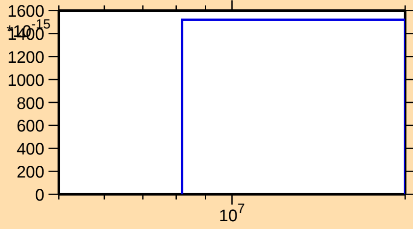
\sigma vs. E for ^{111}\text{Sb}(\text{mt } 34)
