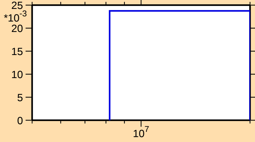
\sigma vs. E for ^{111}\text{Sb}(n,2n)
