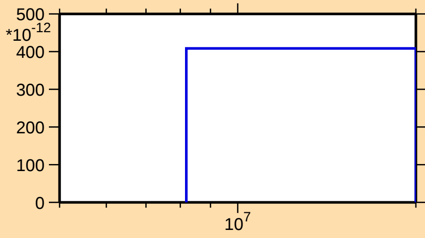
\sigma vs. E for ^{111}\text{Sb}(n,\text{pt})
