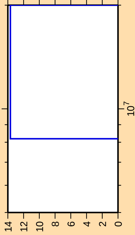
\Delta\sigma/\sigma vs. E for ^{111}\text{Sb}(\text{mt } 34)
