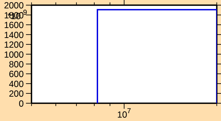
\sigma vs. E for ^{111}\text{Sb}(n,nd)
