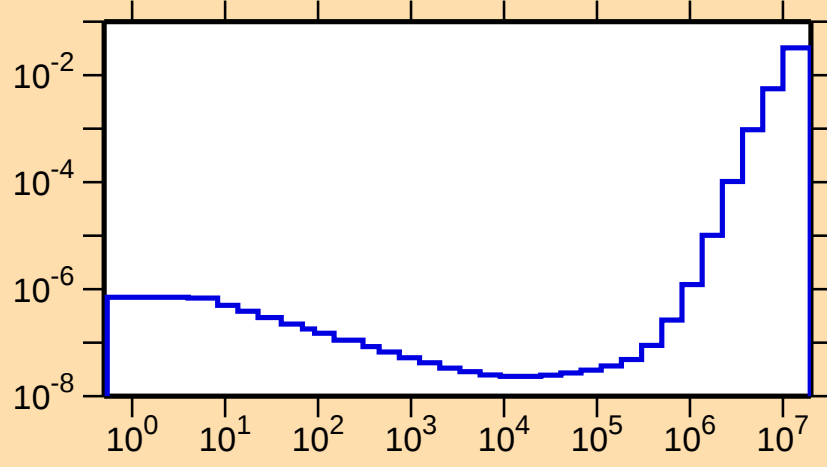
\sigma vs. E for ^{120}\text{Sb}(n,p)
