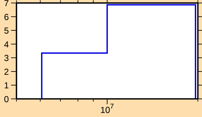
\Delta\sigma/\sigma vs. E for ^{120}\text{Sb}(n,\text{tot.})
