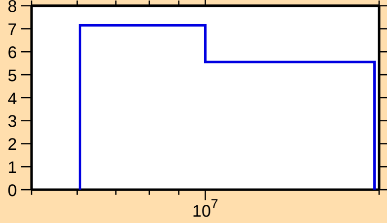
\Delta\sigma/\sigma vs. E for ^{120}\text{Sb}(n,\text{nonel.})
