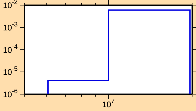
\sigma vs. E for ^{120}\text{Sb}(n,np)
