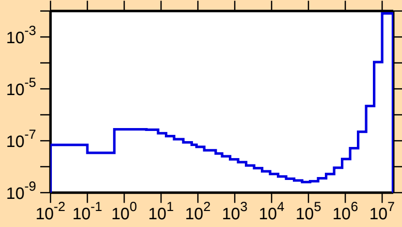
\sigma vs. E for ^{120}\text{Sb}(n,\alpha)
