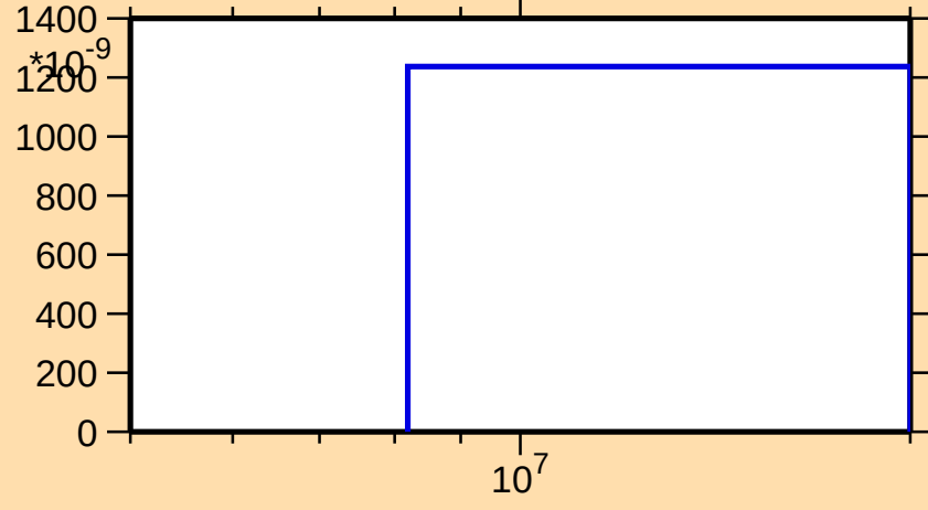
\sigma vs. E for ^{120}\text{Sb}(n,nd)
