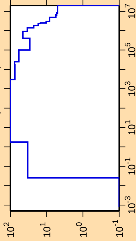
\Delta\sigma/\sigma vs. E for ^{122}\text{Sb}(n,\text{nonel.})
