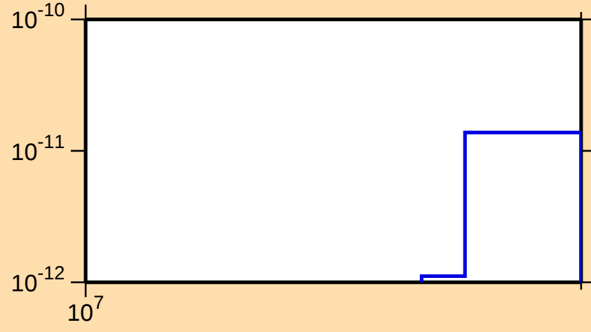
\sigma vs. E for ^{122}\text{Sb}(n,p\alpha)
