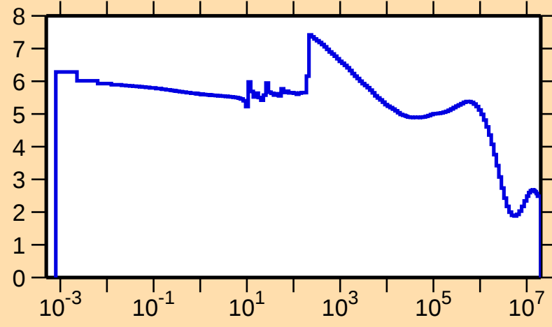
\sigma vs. E for ^{122}\text{Sb}(n,\text{el.})
