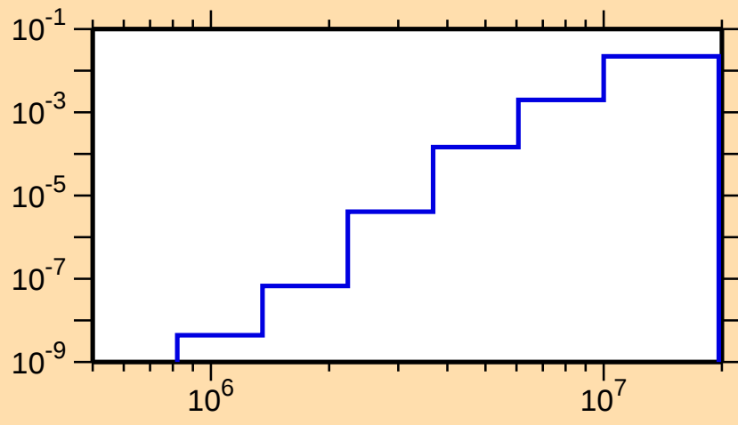
\sigma vs. E for ^{122}\text{Sb}(n,p)
