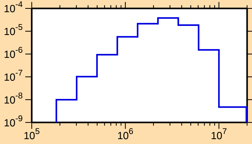
\sigma vs. E for ^{122}\text{Sb}(n,n_4)
