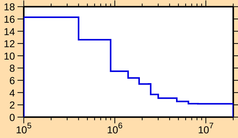
\Delta\sigma/\sigma vs. E for ^{122}\text{Sb}(n,n\text{onel.})
