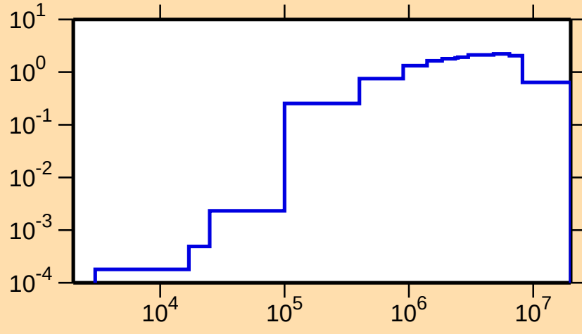
\sigma vs. E for ^{122}\text{Sb}(n,\text{inel.})
