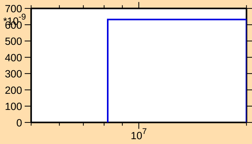
\sigma vs. E for ^{122}\text{Sb}(n,nd)
