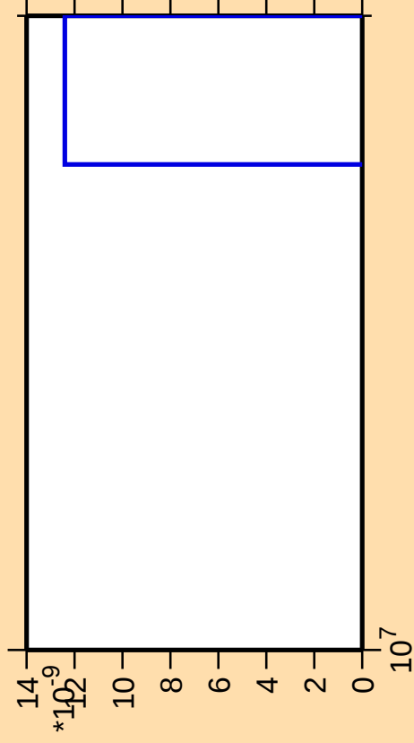
\Delta\sigma/\sigma vs. E for ^{123}\text{Sb}(\text{mt } 11)
