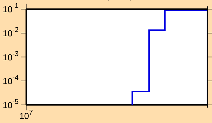
\sigma vs. E for ^{123}\text{Sb}(n,3n)
