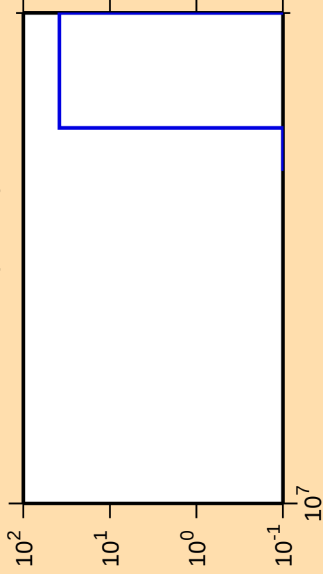
\Delta\sigma/\sigma vs. E for ^{123}\text{Sb}(n,2n\alpha)
