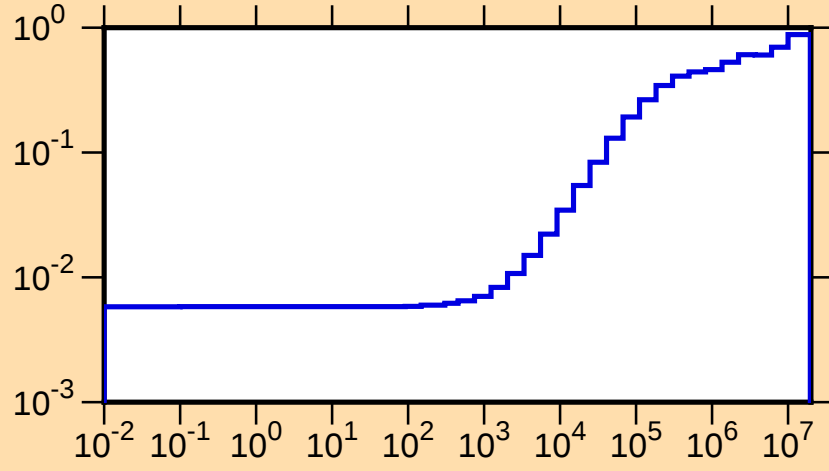
\mu vs. E for ^{123}\text{Sb}(\text{mt251})
