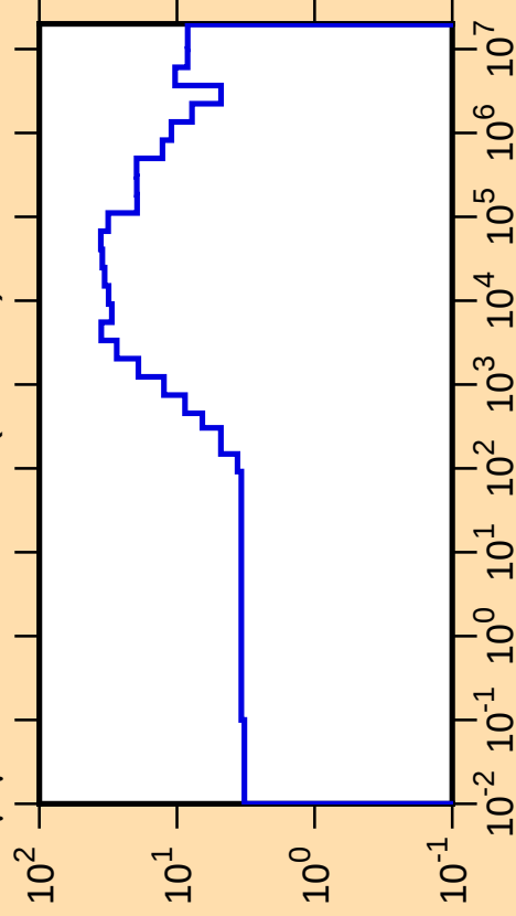
\Delta\mu/\mu vs. E for ^{123}\text{Sb}(\text{mt251})
