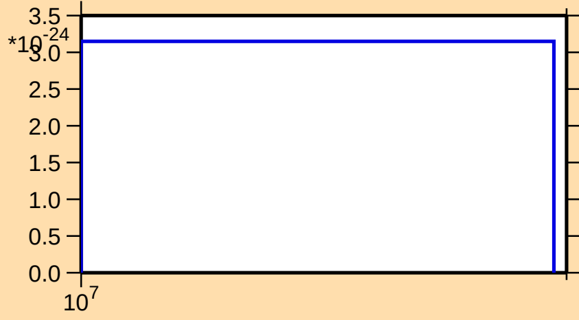
\sigma vs. E for ^{123}\text{Sb}(\text{mt } 11)
