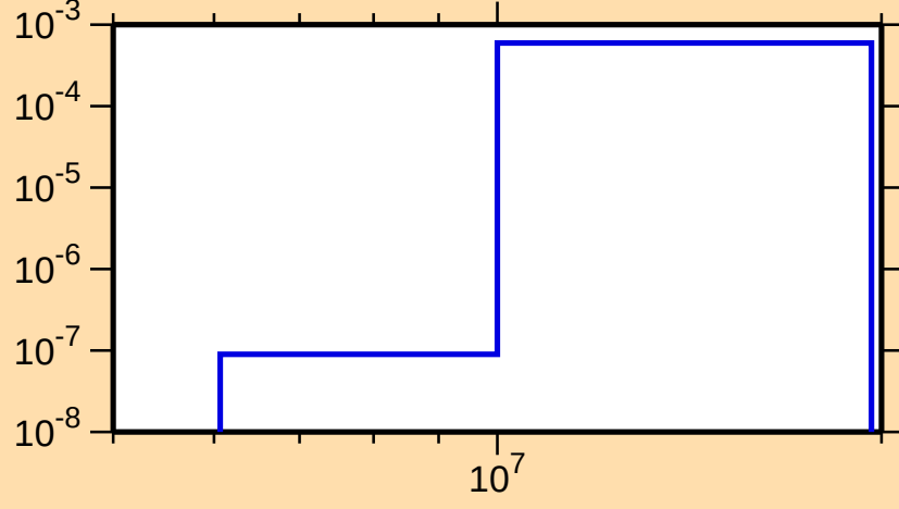
\sigma vs. E for ^{123}\text{Sb}(n,np)
