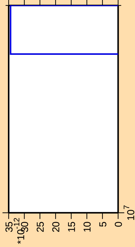
\Delta\sigma/\sigma vs. E for ^{127}\text{Sb}(\text{mt } 11)
