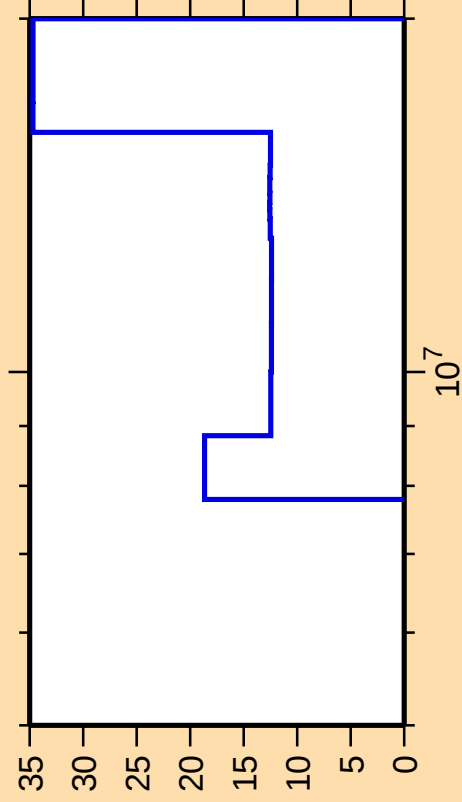
\Delta\sigma/\sigma vs. E for ^{127}\text{Sb}(n,2n)
