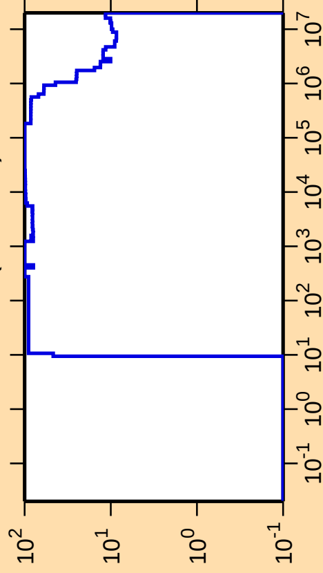
\Delta\sigma/\sigma vs. E for ^{127}\text{Sb}(n,\text{nonel.})
