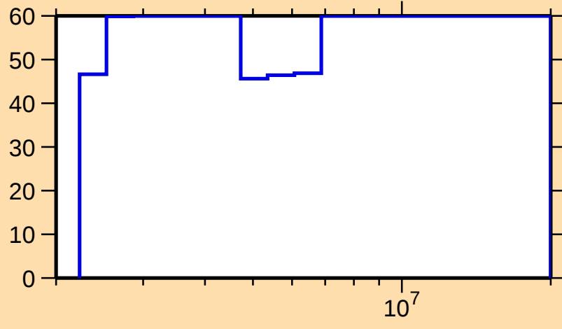
\Delta\sigma/\sigma vs. E for ^{127}\text{Sb}(n,n_1)
