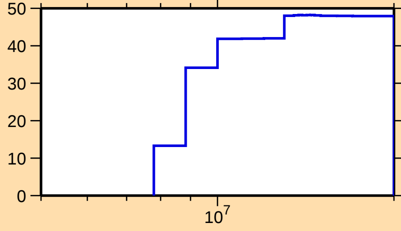
\Delta\sigma/\sigma vs. E for ^{127}\text{Sb}(n,\text{inel.})
