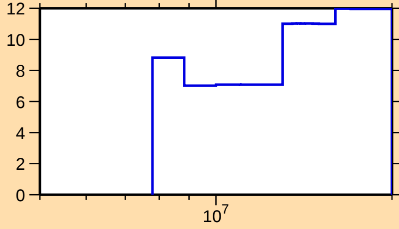
\Delta\sigma/\sigma vs. E for ^{127}\text{Sb}(n,\text{tot.})
