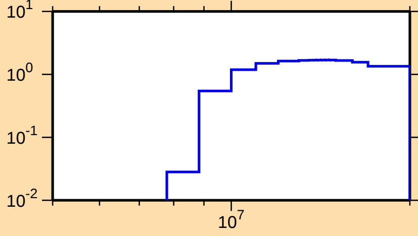
\sigma vs. E for ^{127}\text{Sb}(n,2n)
