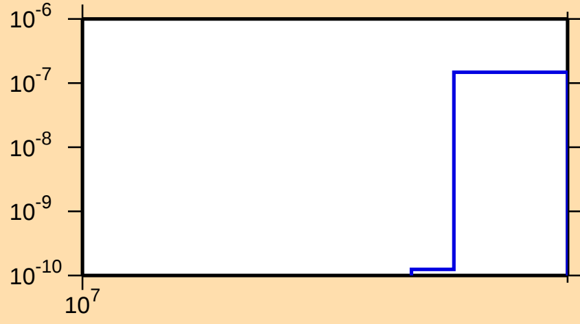
\sigma vs. E for ^{127}\text{Sb}(n,nt)
