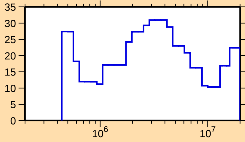
\Delta\sigma/\sigma vs. E for ^{127}\text{Sb}(n,\text{el.})
