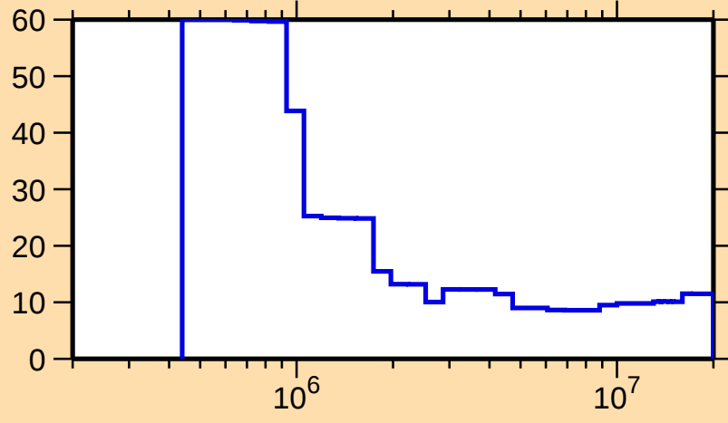
\Delta\sigma/\sigma vs. E for ^{127}\text{Sb}(n,\text{nonel.})
