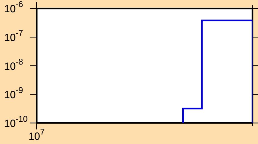
\sigma vs. E for ^{127}\text{Sb}(n,\text{nd})
