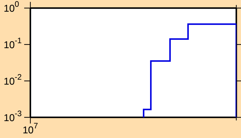
\sigma vs. E for ^{127}\text{Sb}(n,3n)
