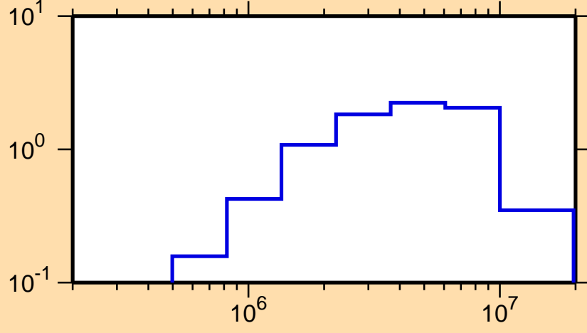
\sigma vs. E for ^{127}\text{Sb}(n,\text{inel.})
