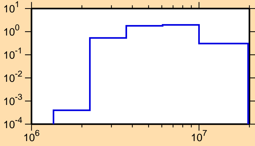
\sigma vs. E for ^{127}\text{Sb}(n,ncont.)
