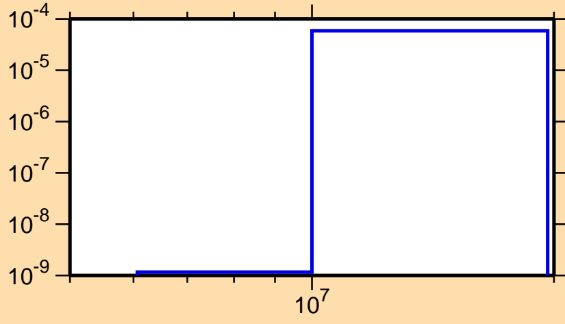
\sigma vs. E for ^{127}\text{Sb}(n,\alpha)
