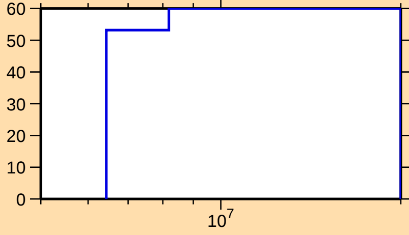
\Delta\sigma/\sigma vs. E for ^{127}\text{Sb}(n,n_1)
