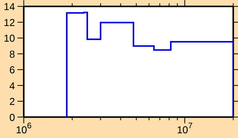
\Delta\sigma/\sigma vs. E for ^{127}\text{Sb}(n,n\text{oncl.})
