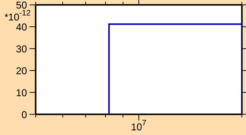
\sigma vs. E for ^{127}\text{Sb}(n,2np)
