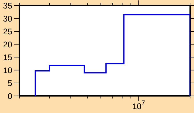
\Delta\sigma/\sigma vs. E for ^{127}\text{Sb}(n,\text{inel.})
