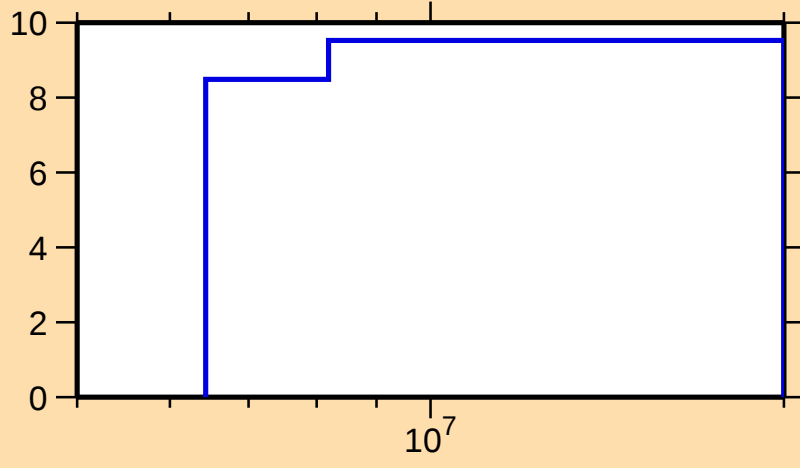
\Delta\sigma/\sigma vs. E for ^{127}\text{Sb}(n,\text{nonel.})
