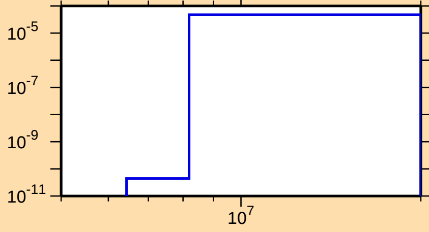
\sigma vs. E for ^{127}\text{Sb}(n,\alpha)
