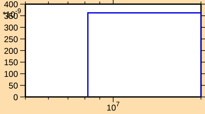
\sigma vs. E for ^{127}\text{Sb}(n,n\alpha)
