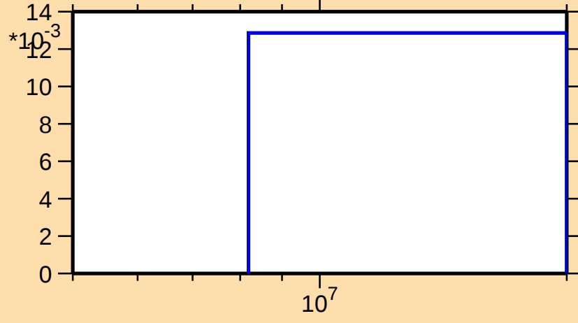
\sigma vs. E for ^{127}\text{Sb}(n,3n)
