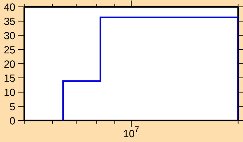
\Delta\sigma/\sigma vs. E for ^{127}\text{Sb}(n,n\text{cont.})
