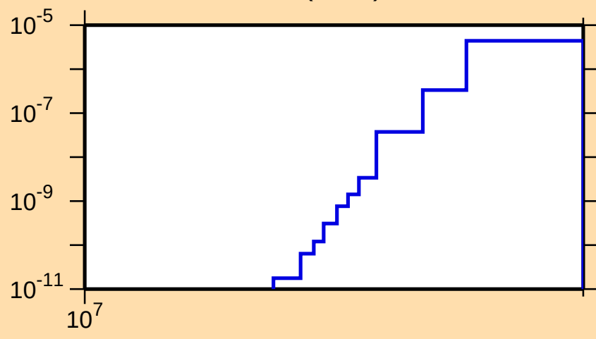
\sigma vs. E for ^{129}\text{Sb}(n,n\alpha)
