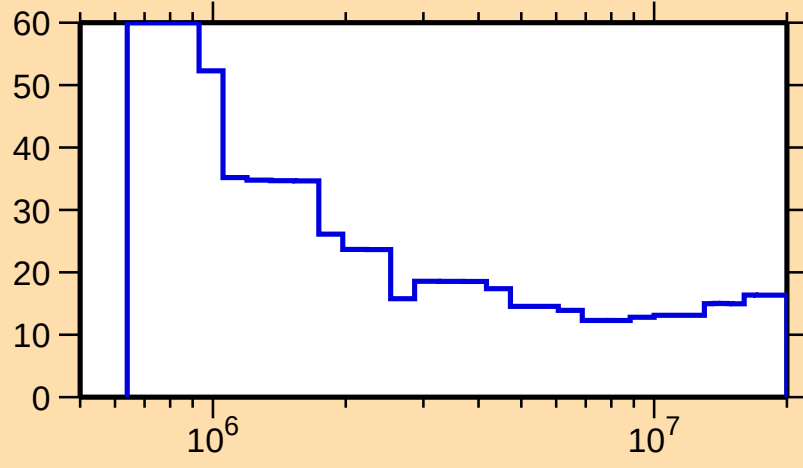
\Delta\sigma/\sigma vs. E for ^{129}\text{Sb}(n,\text{nonel.})
