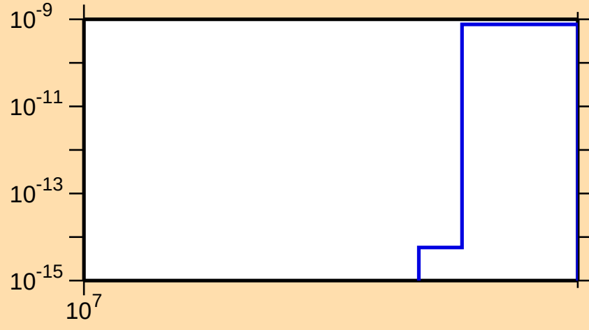
\sigma vs. E for ^{129}\text{Sb}(n,2np)
