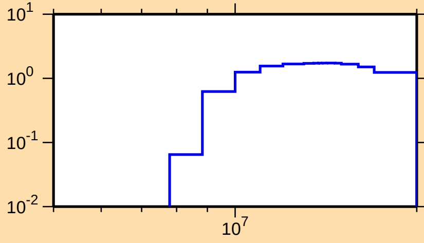
\sigma vs. E for ^{129}\text{Sb}(n,2n)
