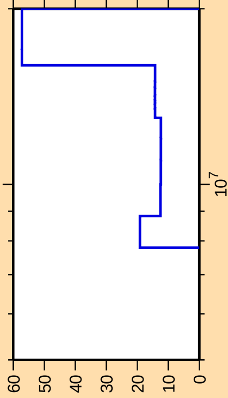
\Delta\sigma/\sigma vs. E for ^{129}\text{Sb}(n,2n)
