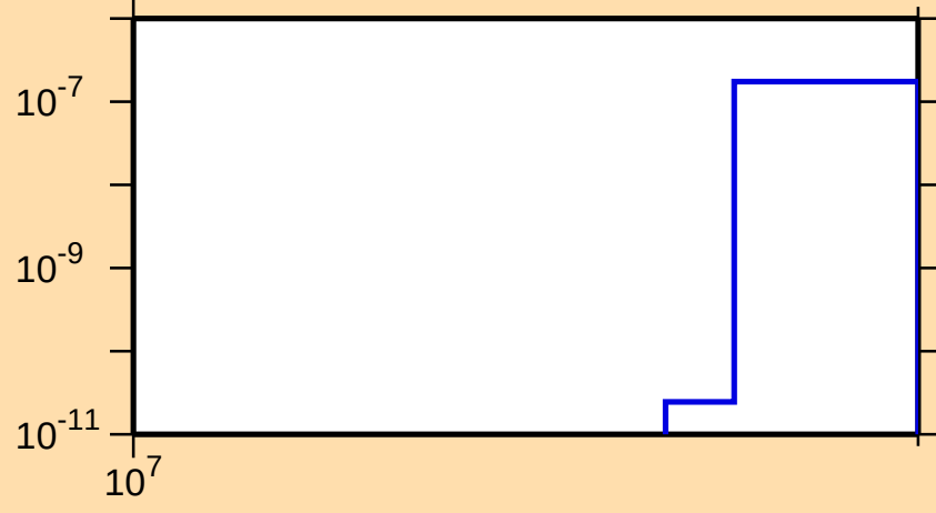
\sigma vs. E for ^{129}\text{Sb}(n,\text{nd})
