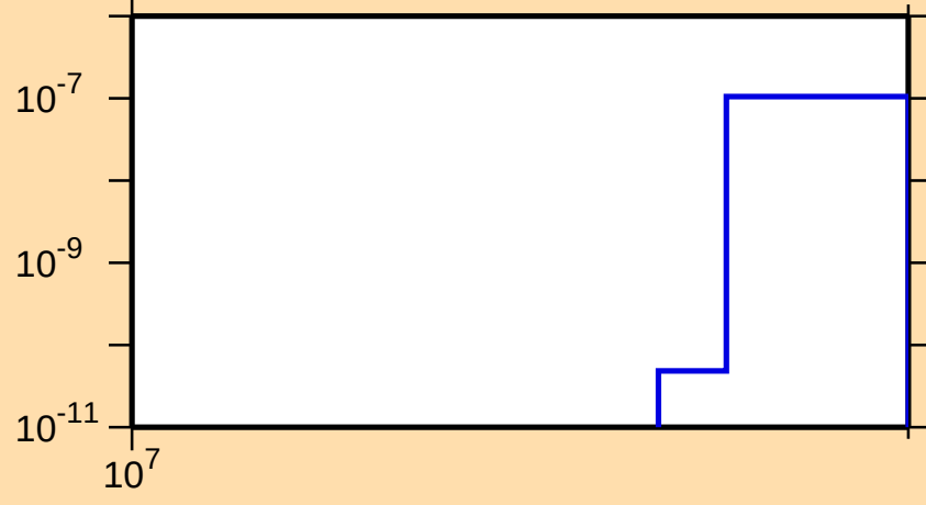
\sigma vs. E for ^{129}\text{Sb}(n,nt)
