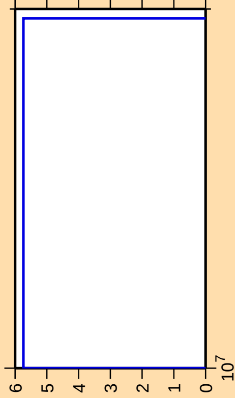
\Delta\sigma/\sigma vs. E for ^{129}\text{Sb}(n,2np)
