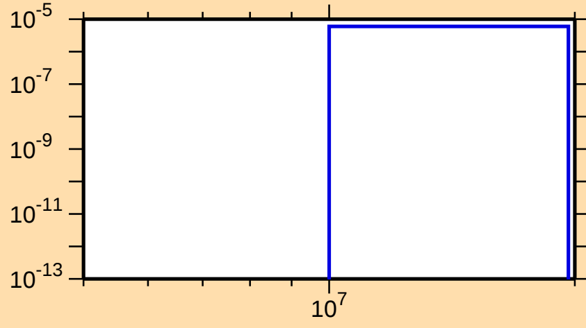
\sigma vs. E for ^{129}\text{Sb}(n,t)
