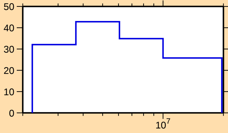
\Delta\sigma/\sigma vs. E for ^{129}\text{Sb}(n,\text{el.})
