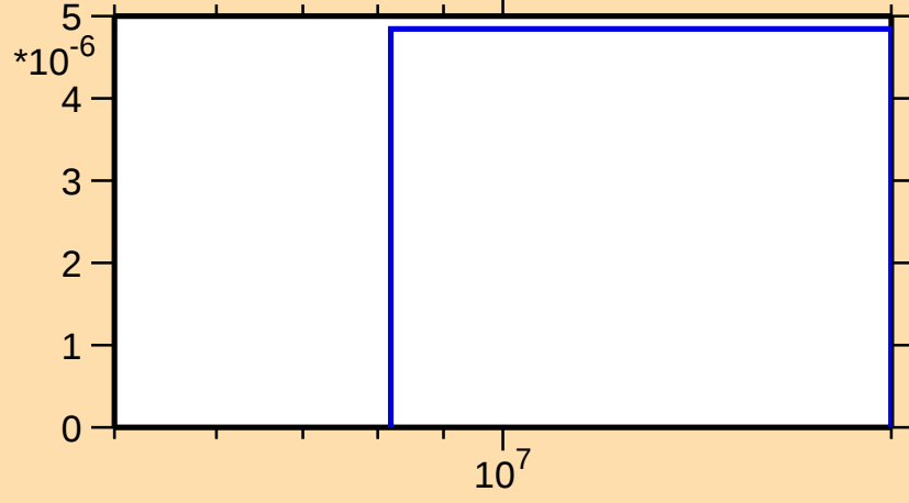
\sigma vs. E for ^{129}\text{Sb}(n,t)
