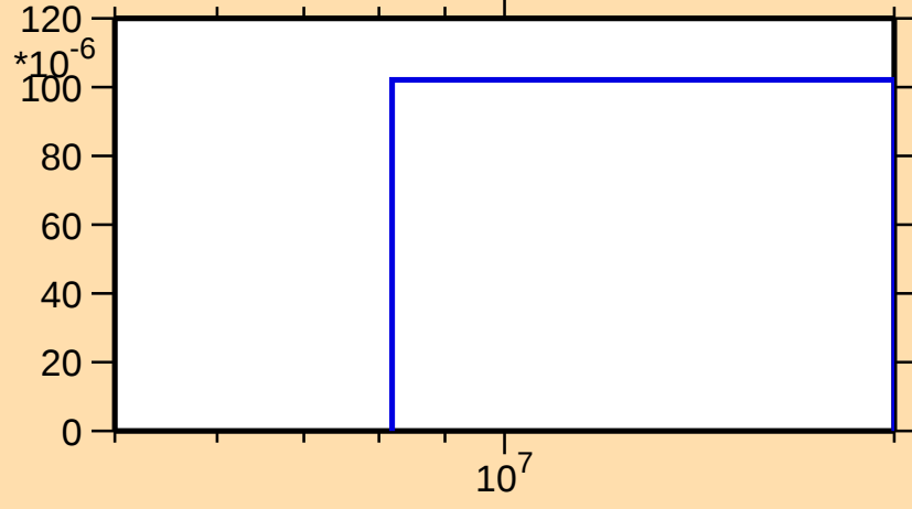
\sigma vs. E for ^{129}\text{Sb}(n,np)
