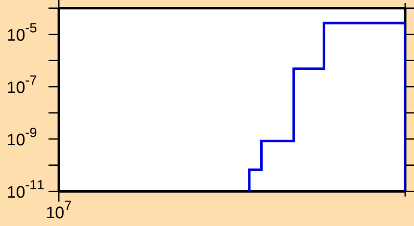
\sigma vs. E for ^{48}\text{Sc}(n,\text{nd})
